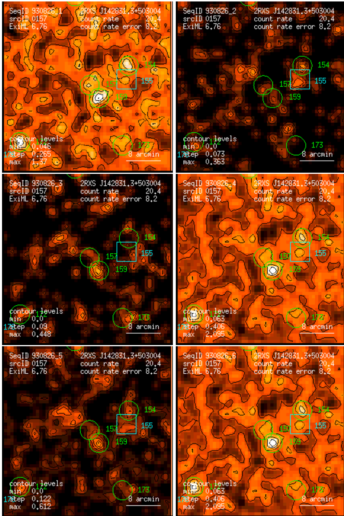
Figure 157: RASS 930826: detection 0157: band rate images, Gaussian filter: (1) PSPC channels 11 – 41, (2) 52 – 90, (3) 91 – 201, (4) 11 – 235, (5) 52 – 201, (6) 11 – 201. Broad band rates in counts/ks. Band rate contour levels in counts/ks/arcmin 2 .
