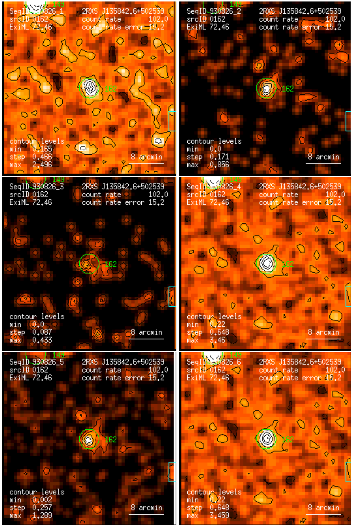
Figure 162: RASS 930826: detection 0162: band rate images, Gaussian filter: (1) PSPC channels 11 – 41, (2) 52 – 90, (3) 91 – 201, (4) 11 – 235, (5) 52 – 201, (6) 11 – 201. Broad band rates in counts/ks. Band rate contour levels in counts/ks/arcmin 2 .
