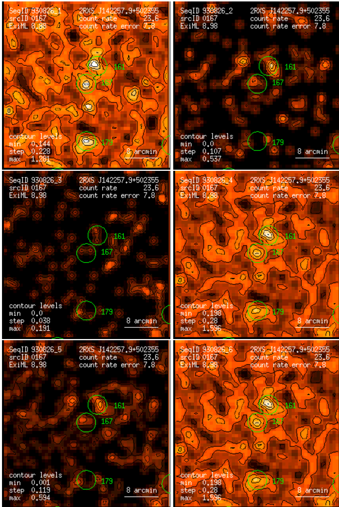
Figure 167: RASS 930826: detection 0167: band rate images, Gaussian filter: (1) PSPC channels 11 – 41, (2) 52 – 90, (3) 91 – 201, (4) 11 – 235, (5) 52 – 201, (6) 11 – 201. Broad band rates in counts/ks. Band rate contour levels in counts/ks/arcmin 2 .
