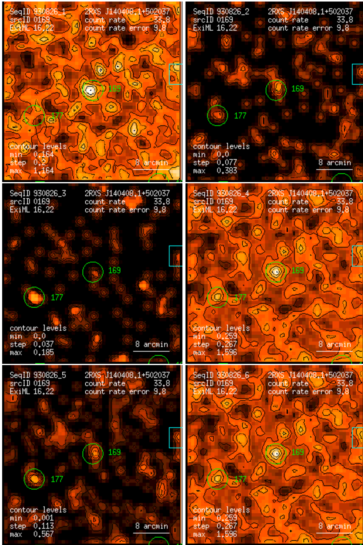
Figure 169: RASS 930826: detection 0169: band rate images, Gaussian filter: (1) PSPC channels 11 – 41, (2) 52 – 90, (3) 91 – 201, (4) 11 – 235, (5) 52 – 201, (6) 11 – 201. Broad band rates in counts/ks. Band rate contour levels in counts/ks/arcmin 2 .
