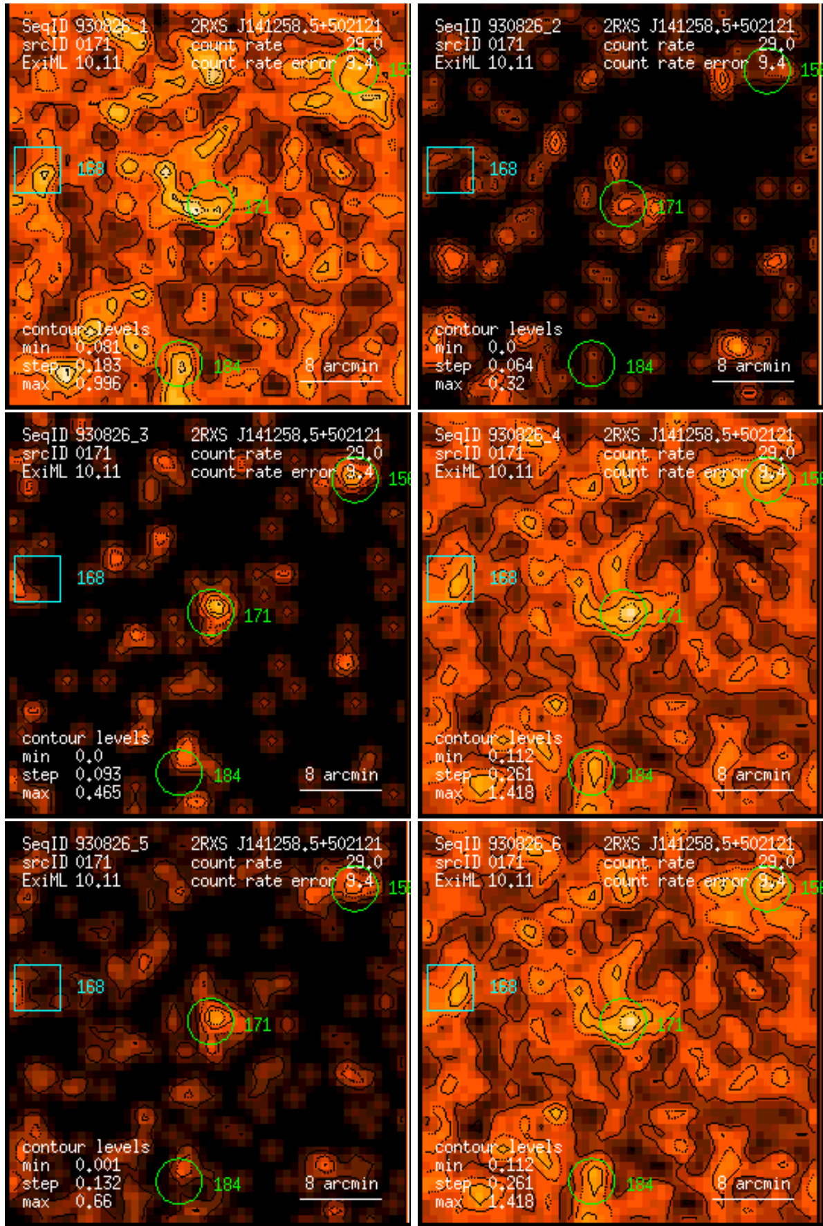
Figure 171: RASS 930826: detection 0171: band rate images, Gaussian filter: (1) PSPC channels 11 – 41, (2) 52 – 90, (3) 91 – 201, (4) 11 – 235, (5) 52 – 201, (6) 11 – 201. Broad band rates in counts/ks. Band rate contour levels in counts/ks/arcmin 2 .
