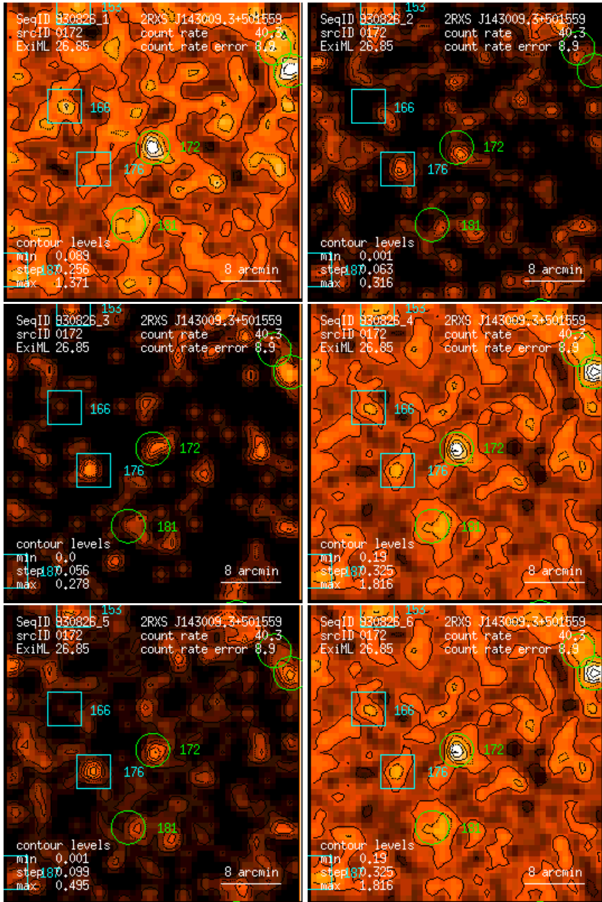
Figure 172: RASS 930826: detection 0172: band rate images, Gaussian filter: (1) PSPC channels 11 – 41, (2) 52 – 90, (3) 91 – 201, (4) 11 – 235, (5) 52 – 201, (6) 11 – 201. Broad band rates in counts/ks. Band rate contour levels in counts/ks/arcmin 2 .
