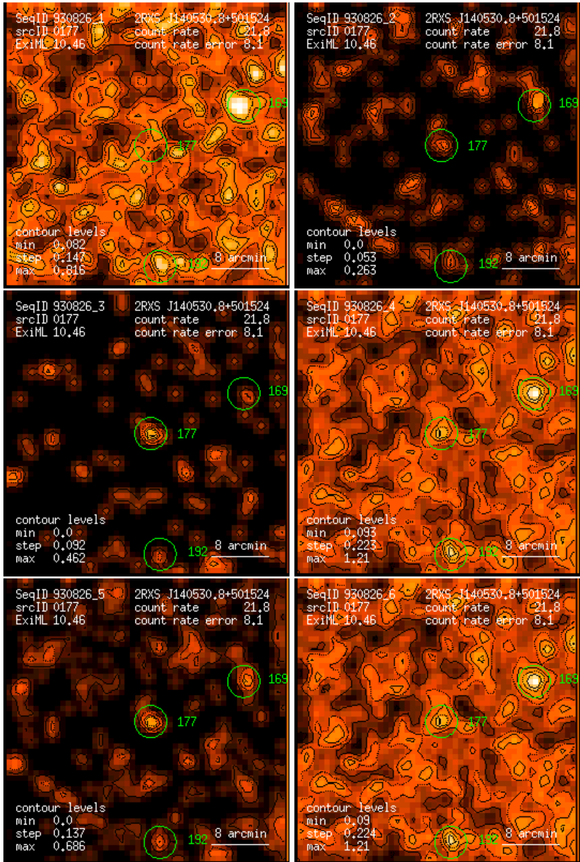
Figure 177: RASS 930826: detection 0177: band rate images, Gaussian filter: (1) PSPC channels 11 – 41, (2) 52 – 90, (3) 91 – 201, (4) 11 – 235, (5) 52 – 201, (6) 11 – 201. Broad band rates in counts/ks. Band rate contour levels in counts/ks/arcmin 2 .
