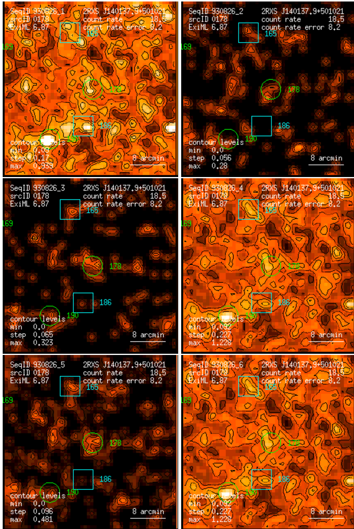
Figure 178: RASS 930826: detection 0178: band rate images, Gaussian filter: (1) PSPC channels 11 – 41, (2) 52 – 90, (3) 91 – 201, (4) 11 – 235, (5) 52 – 201, (6) 11 – 201. Broad band rates in counts/ks. Band rate contour levels in counts/ks/arcmin 2 .
