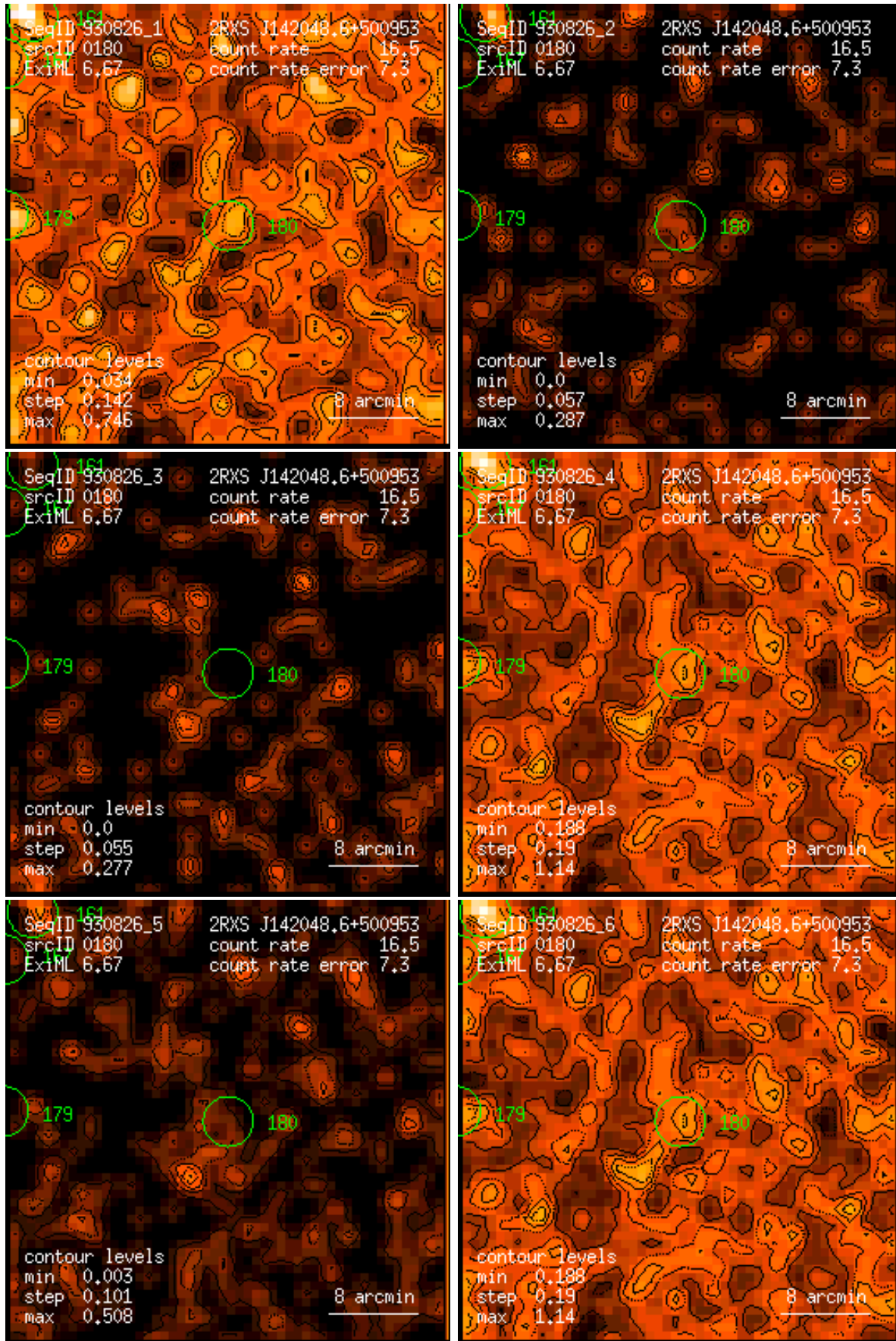
Figure 180: RASS 930826: detection 0180: band rate images, Gaussian filter: (1) PSPC channels 11 – 41, (2) 52 – 90, (3) 91 – 201, (4) 11 – 235, (5) 52 – 201, (6) 11 – 201. Broad band rates in counts/ks. Band rate contour levels in counts/ks/arcmin 2 .
