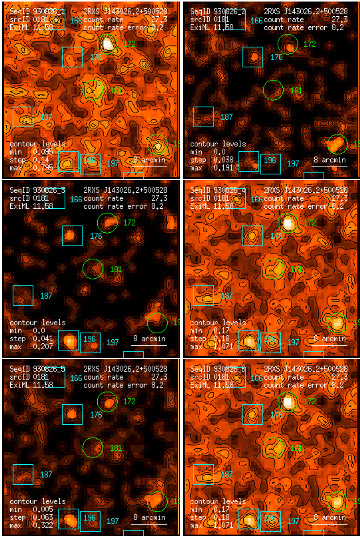
Figure 181: RASS 930826: detection 0181: band rate images, Gaussian filter: (1) PSPC channels 11 – 41, (2) 52 – 90, (3) 91 – 201, (4) 11 – 235, (5) 52 – 201, (6) 11 – 201. Broad band rates in counts/ks. Band rate contour levels in counts/ks/arcmin 2 .
