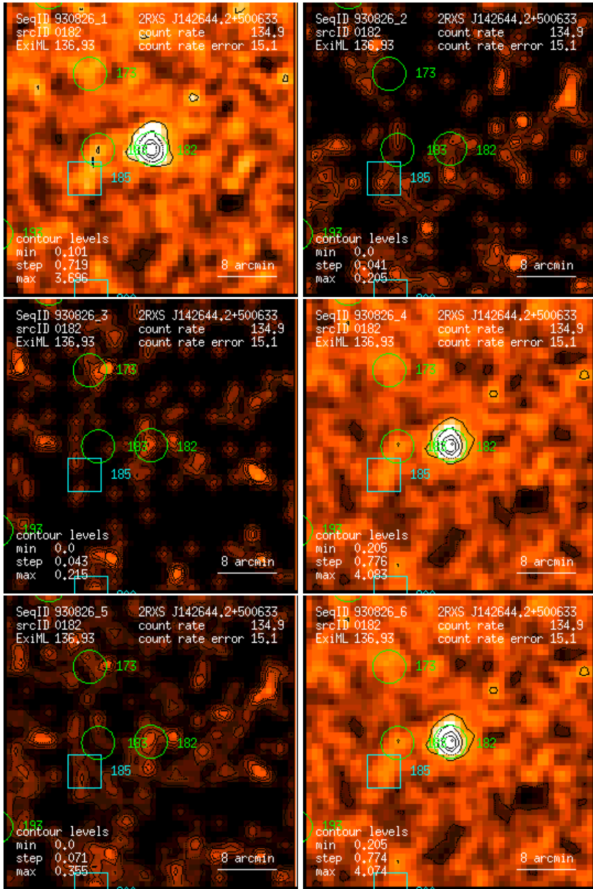
Figure 182: RASS 930826: detection 0182: band rate images, Gaussian filter: (1) PSPC channels 11 – 41, (2) 52 – 90, (3) 91 – 201, (4) 11 – 235, (5) 52 – 201, (6) 11 – 201. Broad band rates in counts/ks. Band rate contour levels in counts/ks/arcmin 2 .
