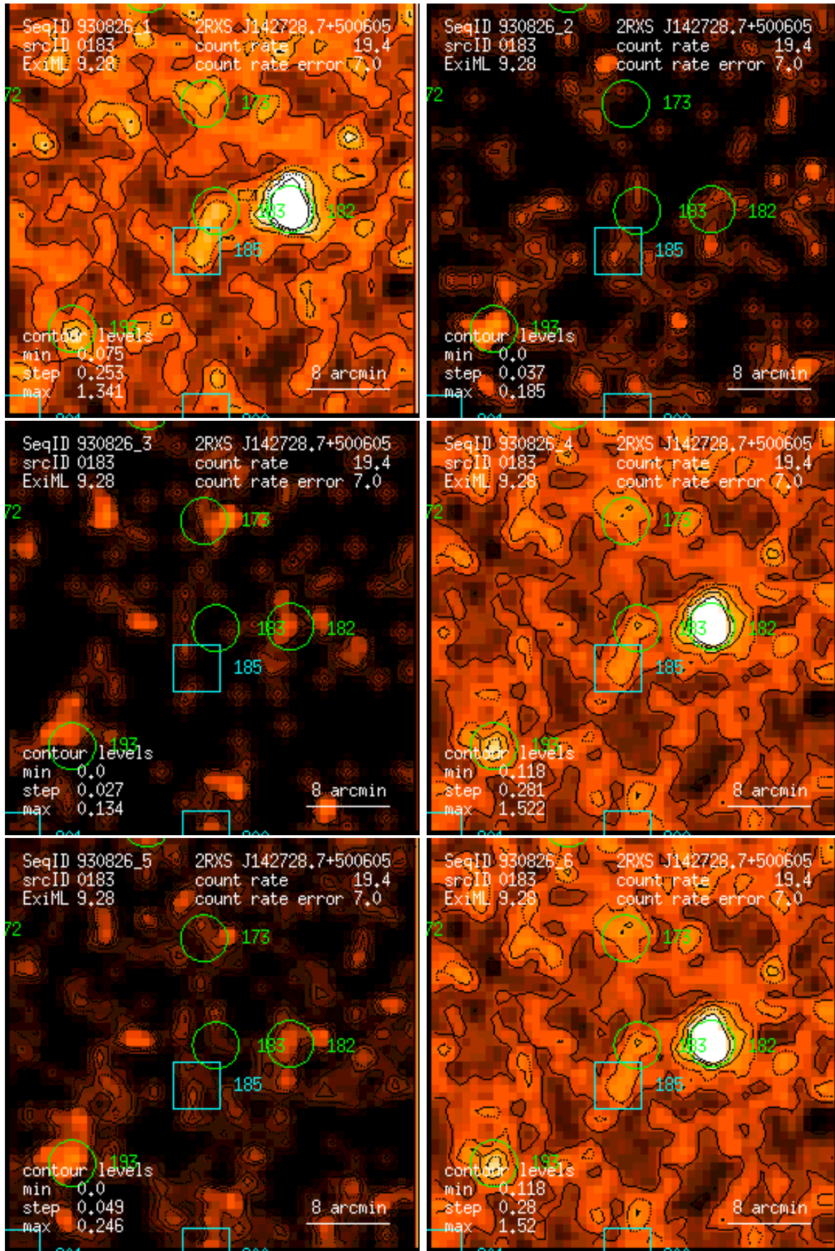
Figure 183: RASS 930826: detection 0183: band rate images, Gaussian filter: (1) PSPC channels 11 – 41, (2) 52 – 90, (3) 91 – 201, (4) 11 – 235, (5) 52 – 201, (6) 11 – 201. Broad band rates in counts/ks. Band rate contour levels in counts/ks/arcmin 2 .
