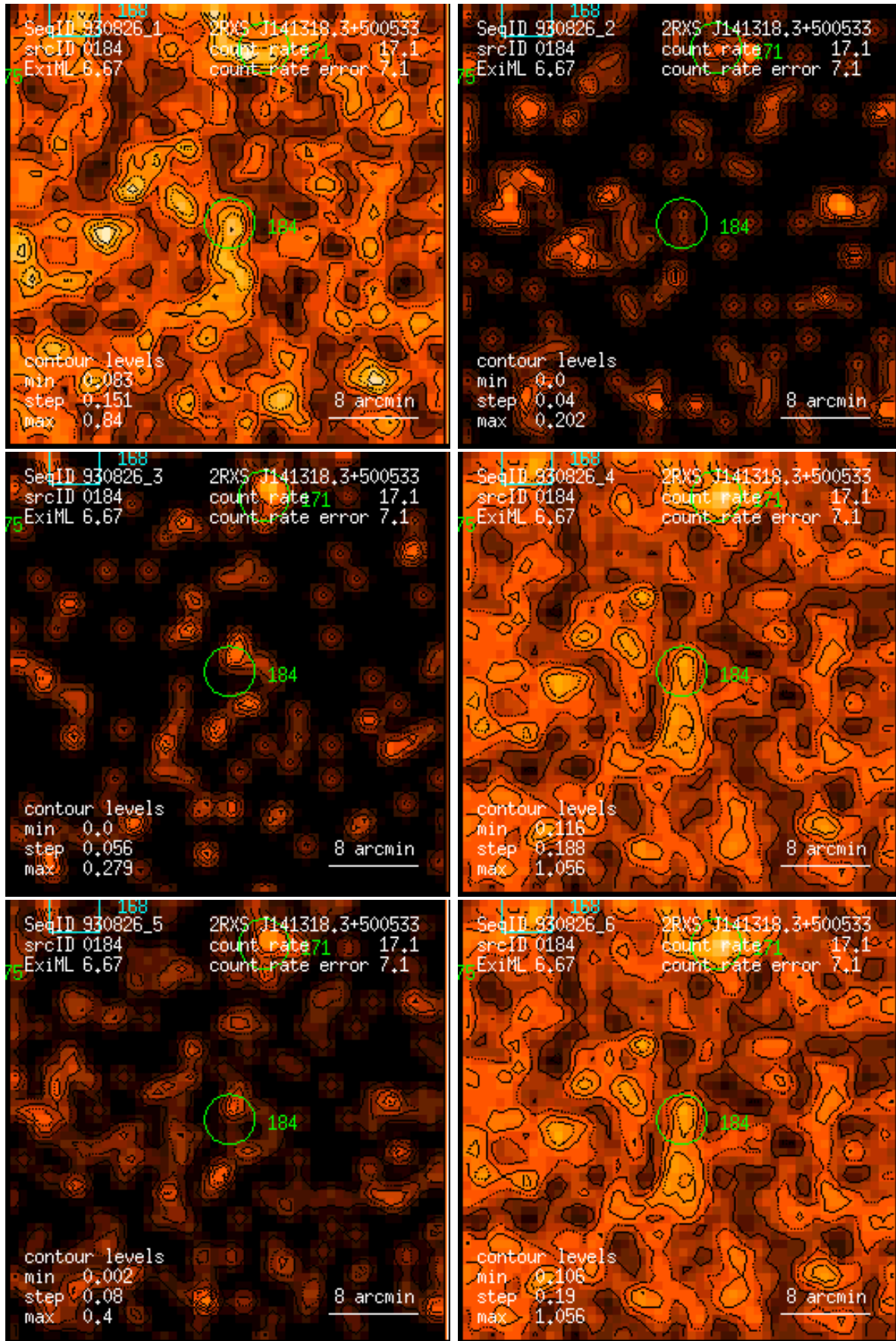
Figure 184: RASS 930826: detection 0184: band rate images, Gaussian filter: (1) PSPC channels 11 – 41, (2) 52 – 90, (3) 91 – 201, (4) 11 – 235, (5) 52 – 201, (6) 11 – 201. Broad band rates in counts/ks. Band rate contour levels in counts/ks/arcmin 2 .
