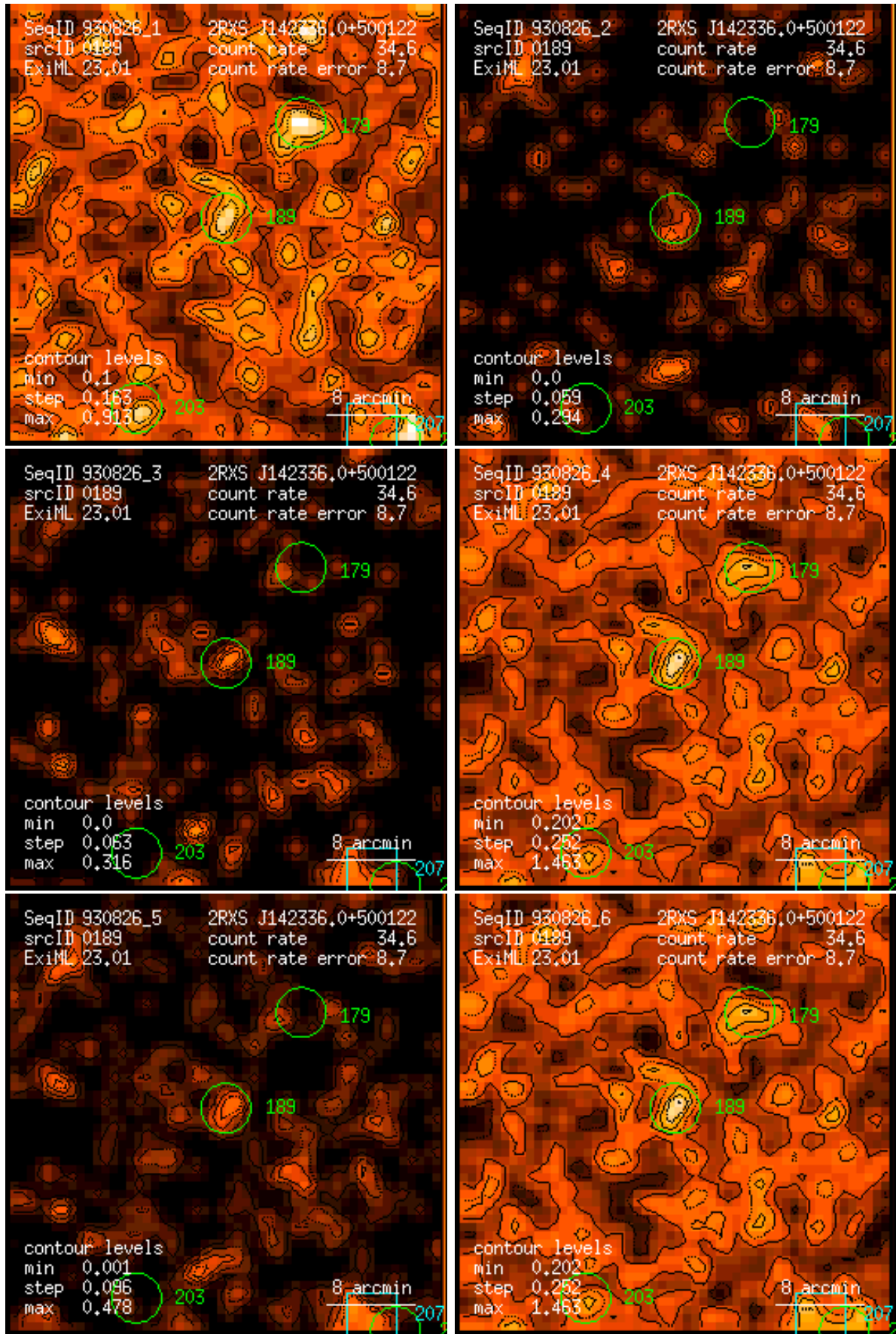
Figure 189: RASS 930826: detection 0189: band rate images, Gaussian filter: (1) PSPC channels 11 – 41, (2) 52 – 90, (3) 91 – 201, (4) 11 – 235, (5) 52 – 201, (6) 11 – 201. Broad band rates in counts/ks. Band rate contour levels in counts/ks/arcmin 2 .
