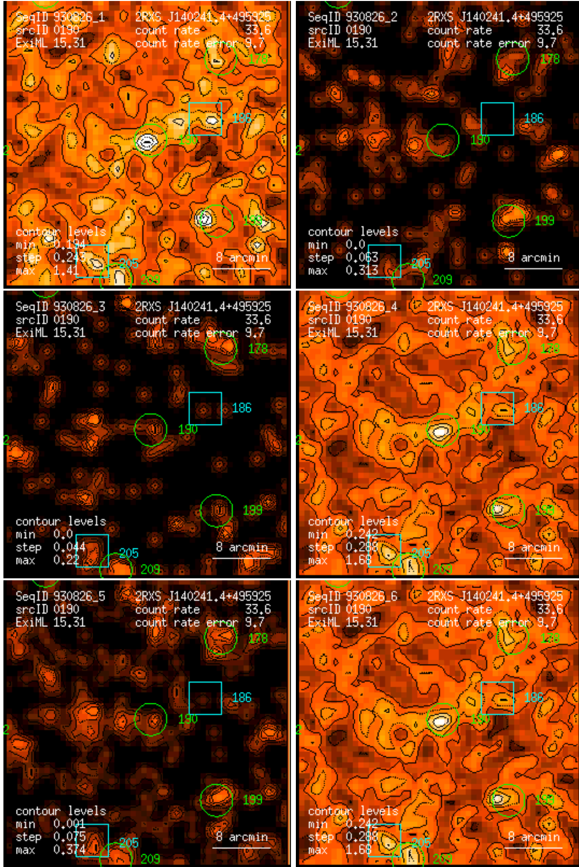
Figure 190: RASS 930826: detection 0190: band rate images, Gaussian filter: (1) PSPC channels 11 – 41, (2) 52 – 90, (3) 91 – 201, (4) 11 – 235, (5) 52 – 201, (6) 11 – 201. Broad band rates in counts/ks. Band rate contour levels in counts/ks/arcmin 2 .
