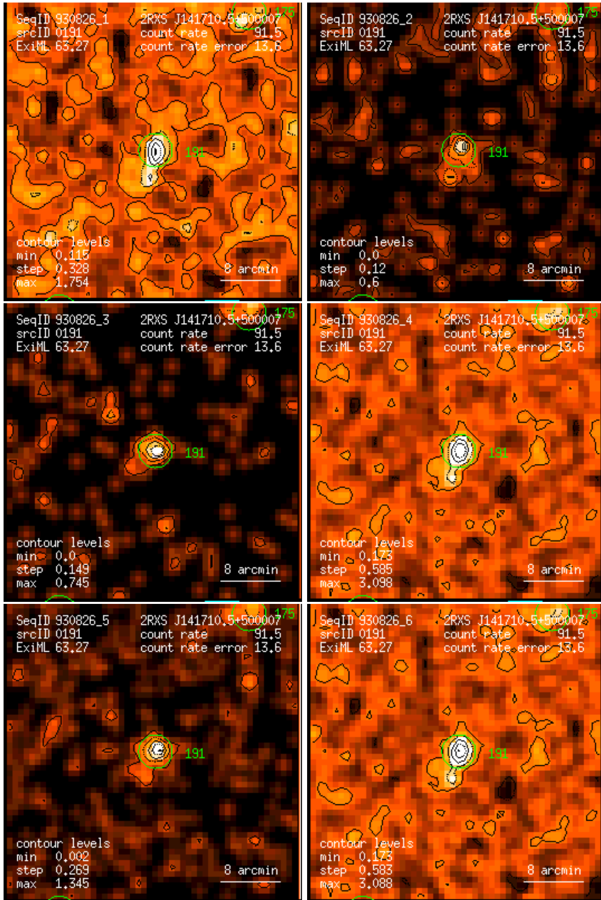
Figure 191: RASS 930826: detection 0191: band rate images, Gaussian filter: (1) PSPC channels 11 – 41, (2) 52 – 90, (3) 91 – 201, (4) 11 – 235, (5) 52 – 201, (6) 11 – 201. Broad band rates in counts/ks. Band rate contour levels in counts/ks/arcmin 2 .
