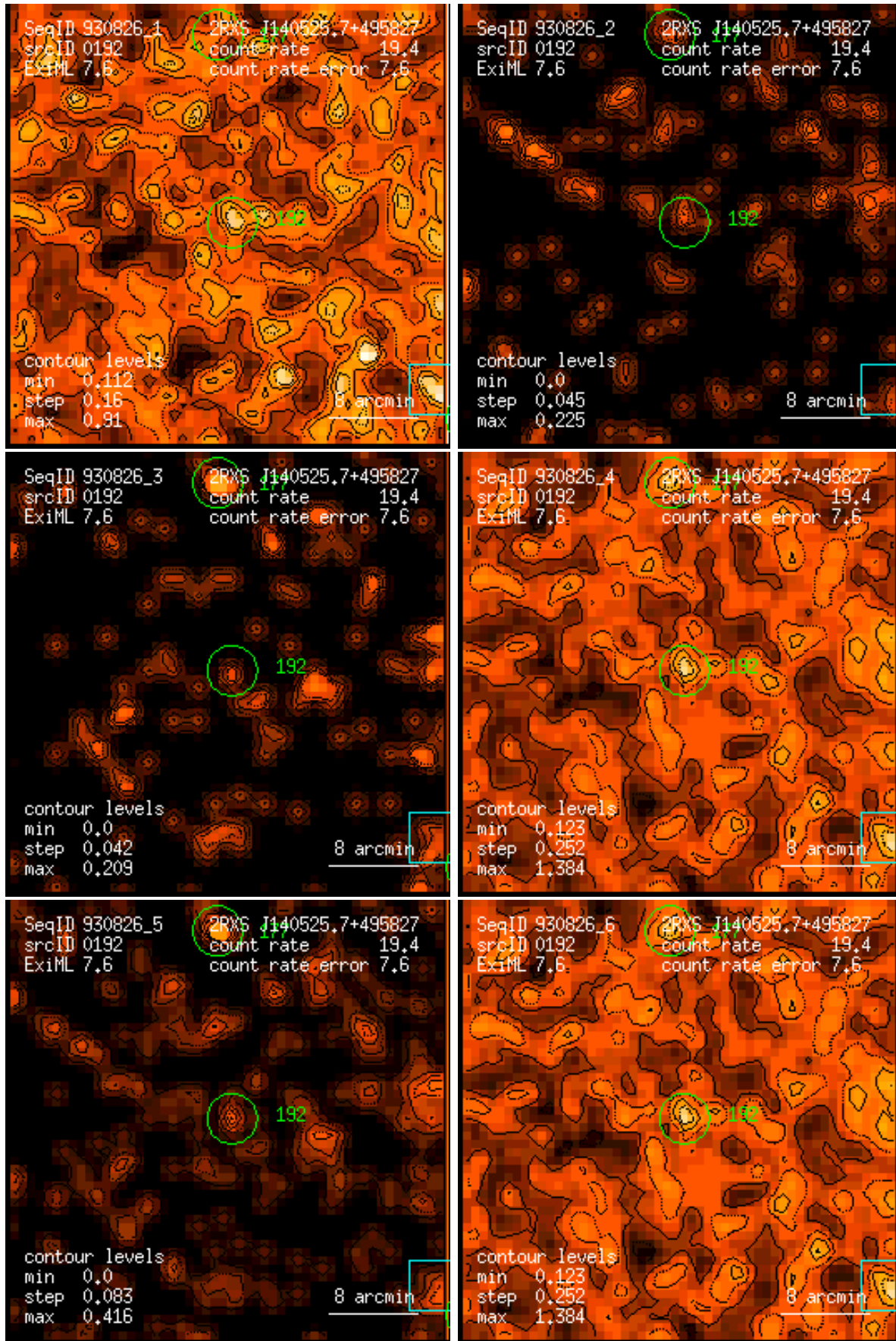
Figure 192: RASS 930826: detection 0192: band rate images, Gaussian filter: (1) PSPC channels 11 – 41, (2) 52 – 90, (3) 91 – 201, (4) 11 – 235, (5) 52 – 201, (6) 11 – 201. Broad band rates in counts/ks. Band rate contour levels in counts/ks/arcmin 2 .
