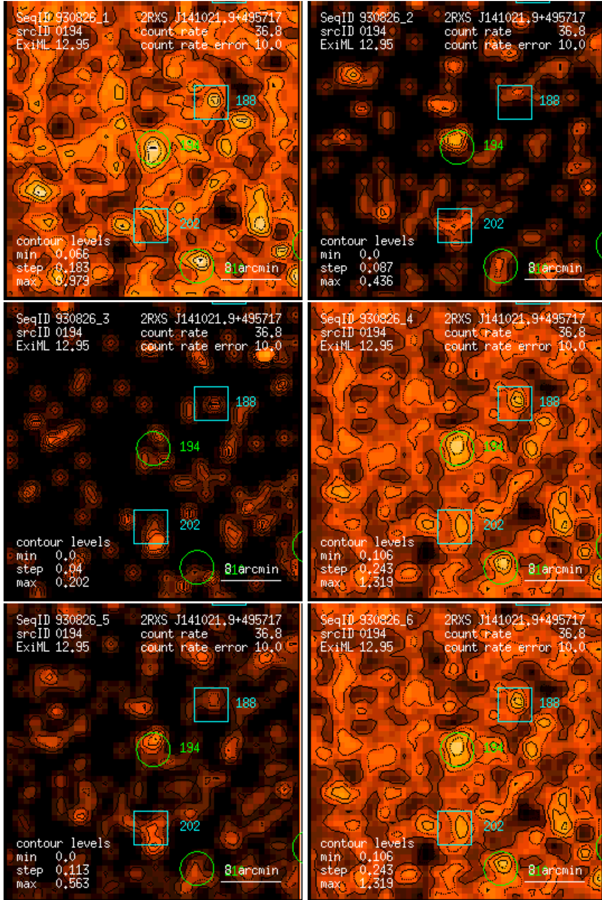
Figure 194: RASS 930826: detection 0194: band rate images, Gaussian filter: (1) PSPC channels 11 – 41, (2) 52 – 90, (3) 91 – 201, (4) 11 – 235, (5) 52 – 201, (6) 11 – 201. Broad band rates in counts/ks. Band rate contour levels in counts/ks/arcmin 2 .
