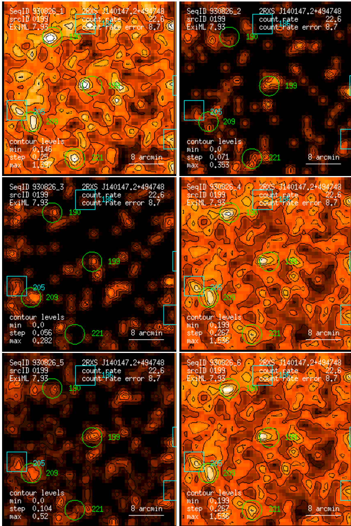
Figure 199: RASS 930826: detection 0199: band rate images, Gaussian filter: (1) PSPC channels 11 – 41, (2) 52 – 90, (3) 91 – 201, (4) 11 – 235, (5) 52 – 201, (6) 11 – 201. Broad band rates in counts/ks. Band rate contour levels in counts/ks/arcmin 2 .
