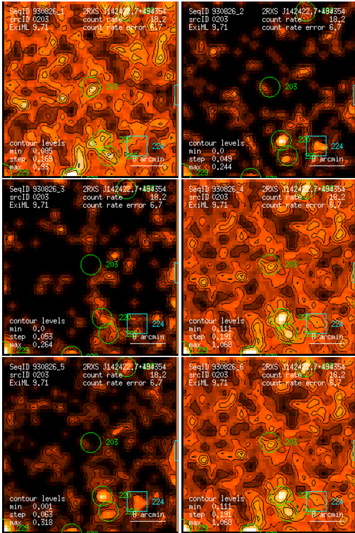
Figure 203: RASS 930826: detection 0203: band rate images, Gaussian filter: (1) PSPC channels 11 – 41, (2) 52 – 90, (3) 91 – 201, (4) 11 – 235, (5) 52 – 201, (6) 11 – 201. Broad band rates in counts/ks. Band rate contour levels in counts/ks/arcmin 2 .
