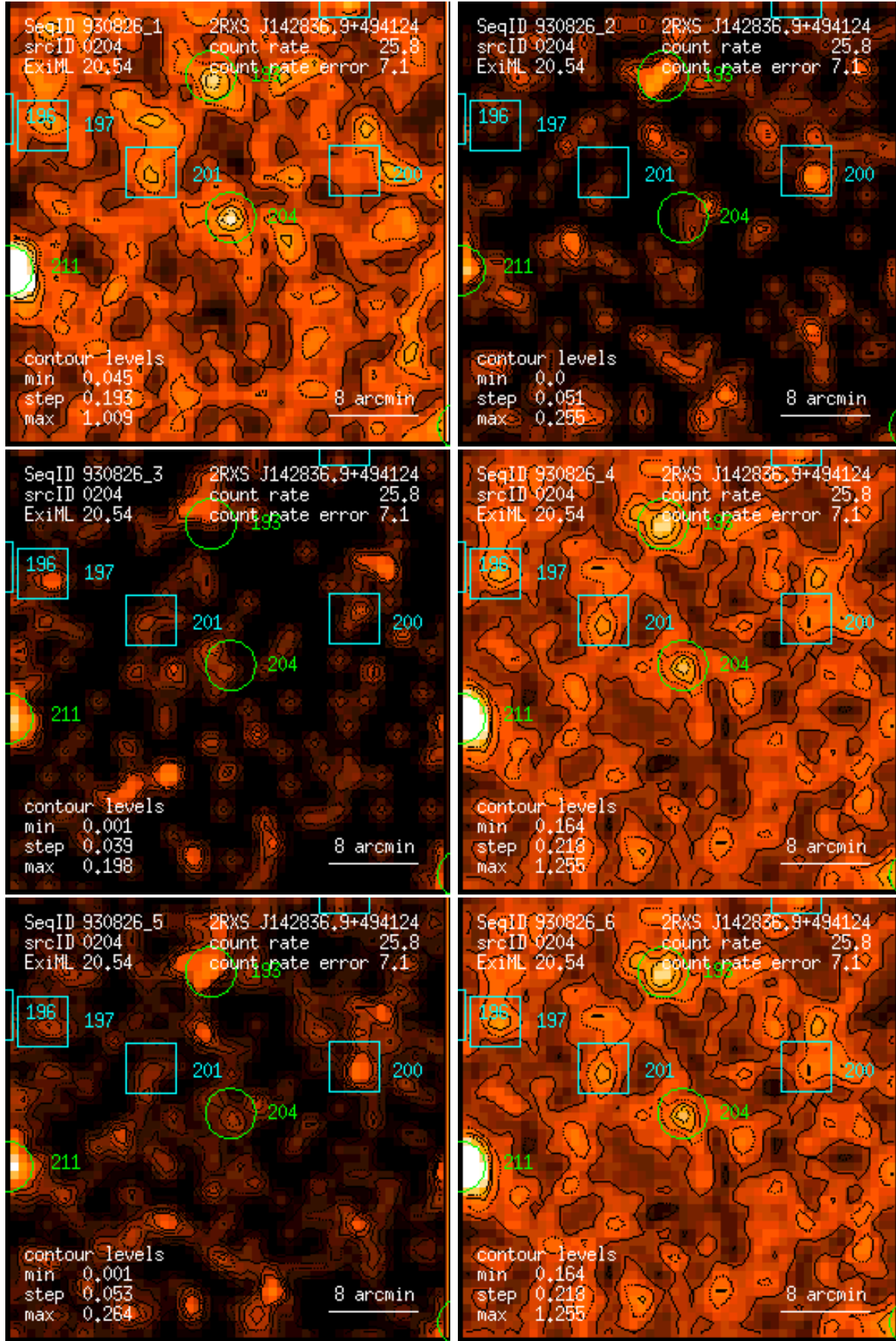
Figure 204: RASS 930826: detection 0204: band rate images, Gaussian filter: (1) PSPC channels 11 – 41, (2) 52 – 90, (3) 91 – 201, (4) 11 – 235, (5) 52 – 201, (6) 11 – 201. Broad band rates in counts/ks. Band rate contour levels in counts/ks/arcmin 2 .
