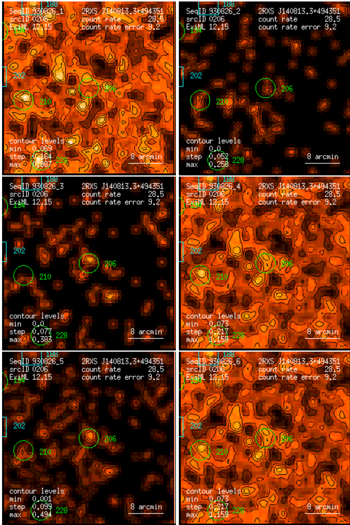
Figure 206: RASS 930826: detection 0206: band rate images, Gaussian filter: (1) PSPC channels 11 – 41, (2) 52 – 90, (3) 91 – 201, (4) 11 – 235, (5) 52 – 201, (6) 11 – 201. Broad band rates in counts/ks. Band rate contour levels in counts/ks/arcmin 2 .
