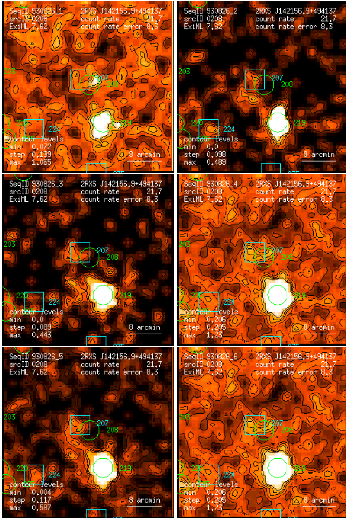
Figure 208: RASS 930826: detection 0208: band rate images, Gaussian filter: (1) PSPC channels 11 – 41, (2) 52 – 90, (3) 91 – 201, (4) 11 – 235, (5) 52 – 201, (6) 11 – 201. Broad band rates in counts/ks. Band rate contour levels in counts/ks/arcmin 2 .
