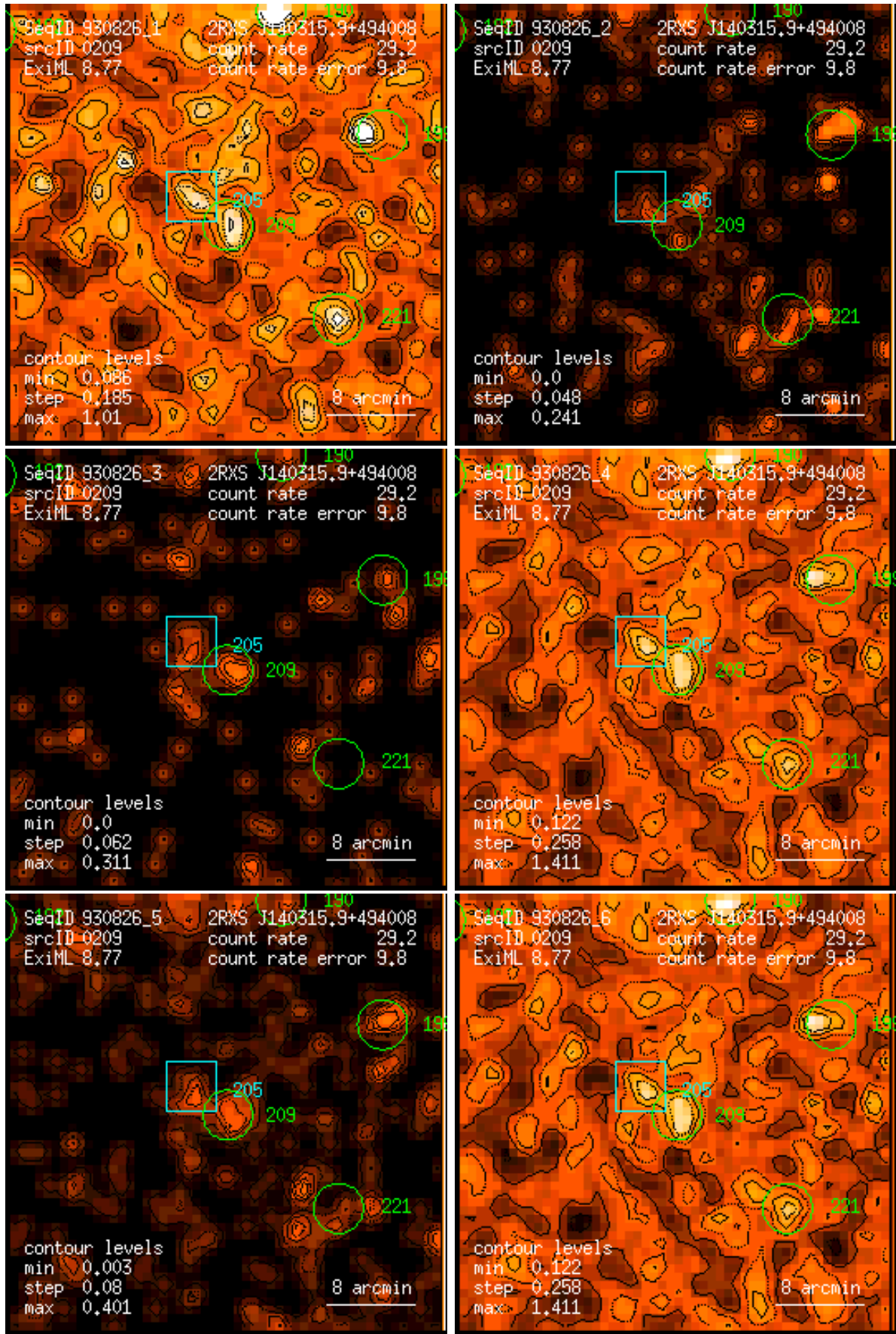
Figure 209: RASS 930826: detection 0209: band rate images, Gaussian filter: (1) PSPC channels 11 – 41, (2) 52 – 90, (3) 91 – 201, (4) 11 – 235, (5) 52 – 201, (6) 11 – 201. Broad band rates in counts/ks. Band rate contour levels in counts/ks/arcmin 2 .
