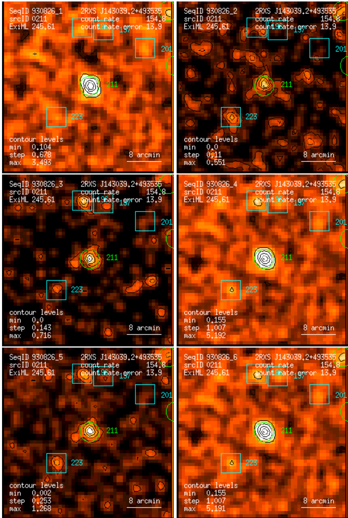
Figure 211: RASS 930826: detection 0211: band rate images, Gaussian filter: (1) PSPC channels 11 – 41, (2) 52 – 90, (3) 91 – 201, (4) 11 – 235, (5) 52 – 201, (6) 11 – 201. Broad band rates in counts/ks. Band rate contour levels in counts/ks/arcmin 2 .
