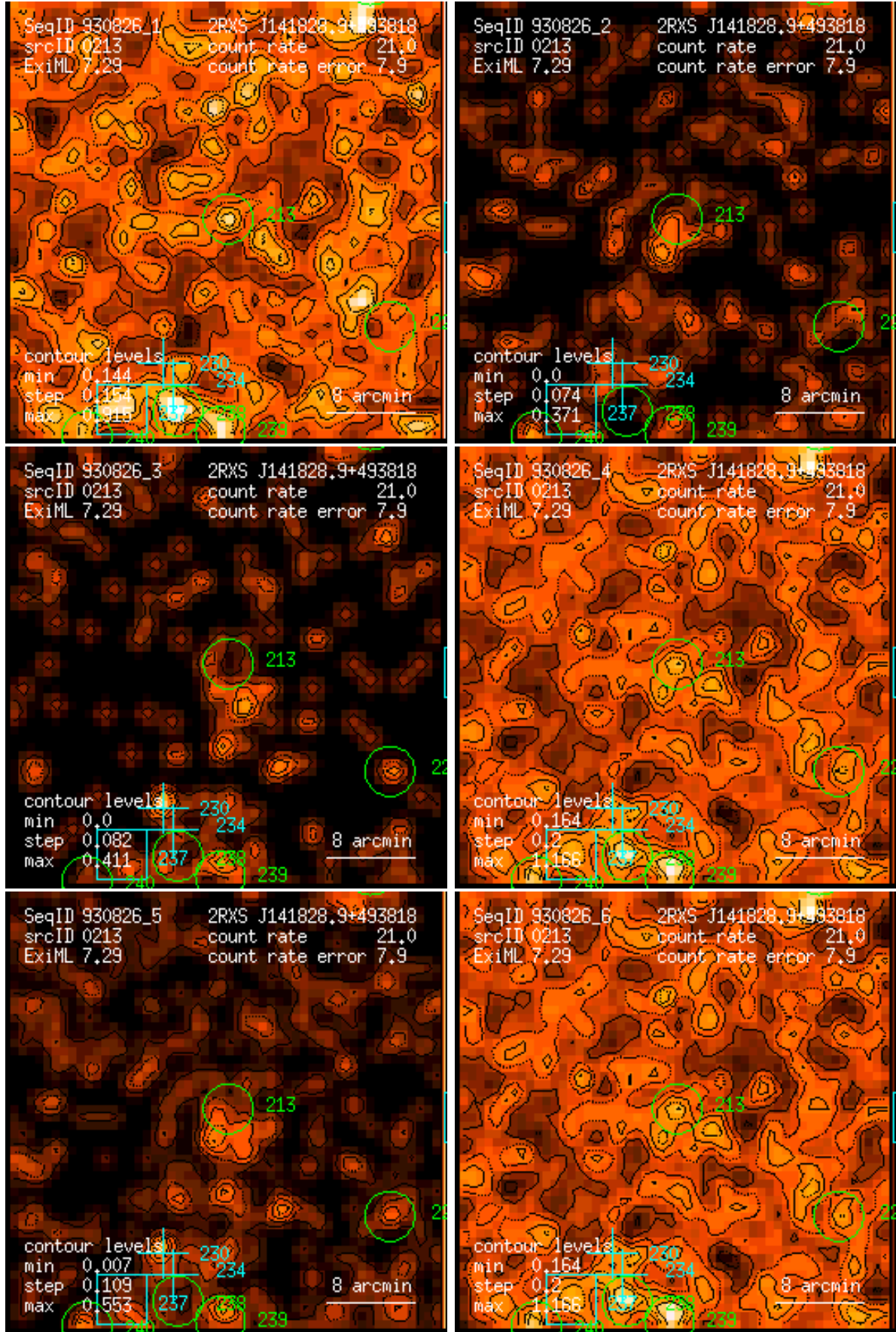
Figure 213: RASS 930826: detection 0213: band rate images, Gaussian filter: (1) PSPC channels 11 – 41, (2) 52 – 90, (3) 91 – 201, (4) 11 – 235, (5) 52 – 201, (6) 11 – 201. Broad band rates in counts/ks. Band rate contour levels in counts/ks/arcmin 2 .
