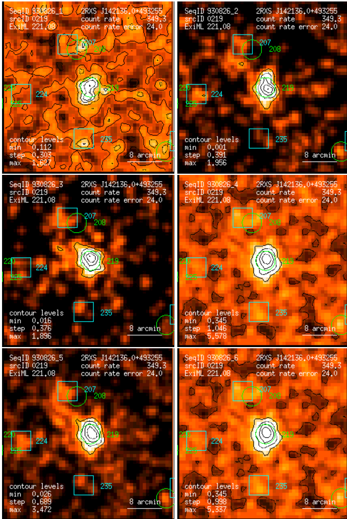
Figure 219: RASS 930826: detection 0219: band rate images, Gaussian filter: (1) PSPC channels 11 – 41, (2) 52 – 90, (3) 91 – 201, (4) 11 – 235, (5) 52 – 201, (6) 11 – 201. Broad band rates in counts/ks. Band rate contour levels in counts/ks/arcmin 2 .
