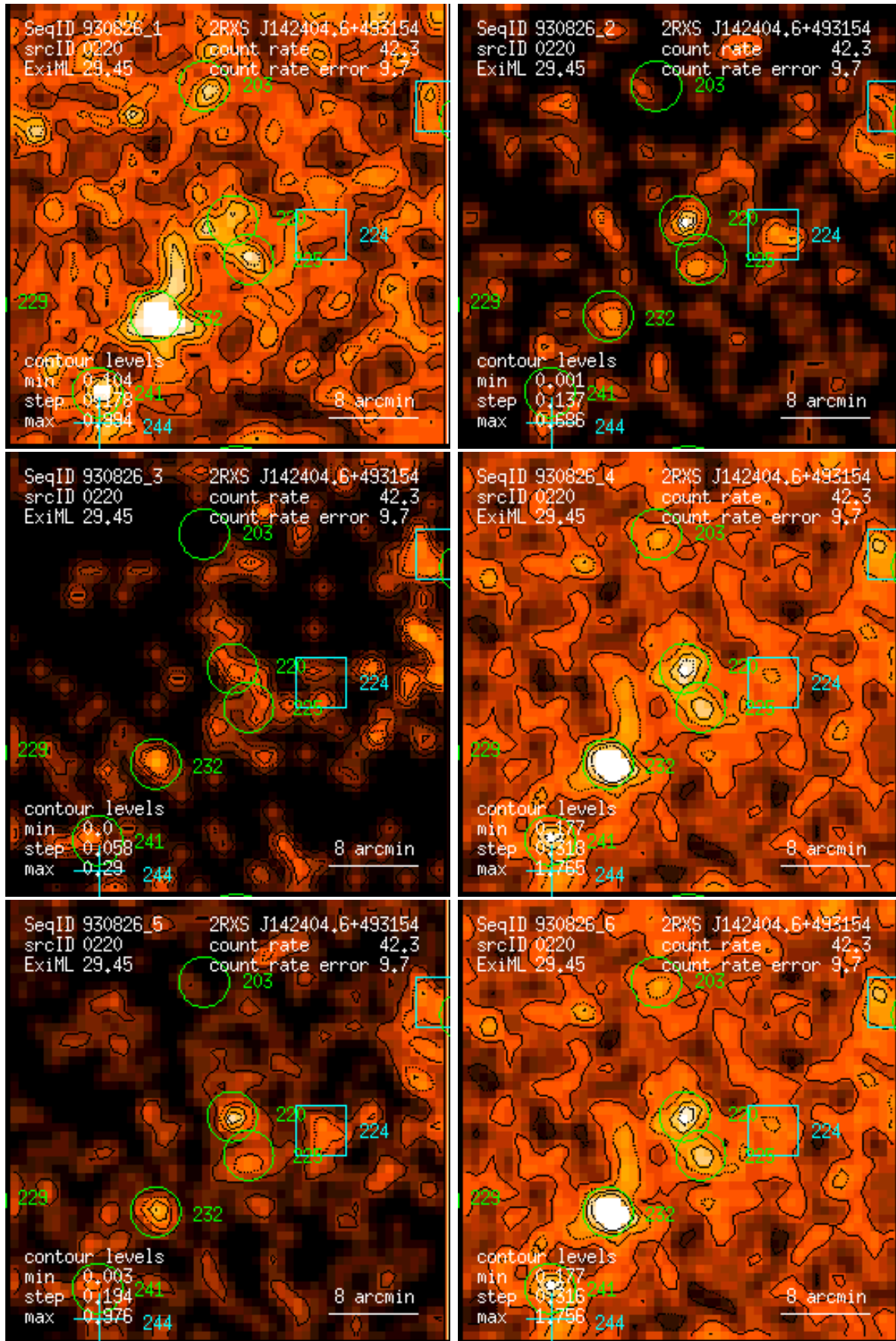
Figure 220: RASS 930826: detection 0220: band rate images, Gaussian filter: (1) PSPC channels 11 – 41, (2) 52 – 90, (3) 91 – 201, (4) 11 – 235, (5) 52 – 201, (6) 11 – 201. Broad band rates in counts/ks. Band rate contour levels in counts/ks/arcmin 2 .
