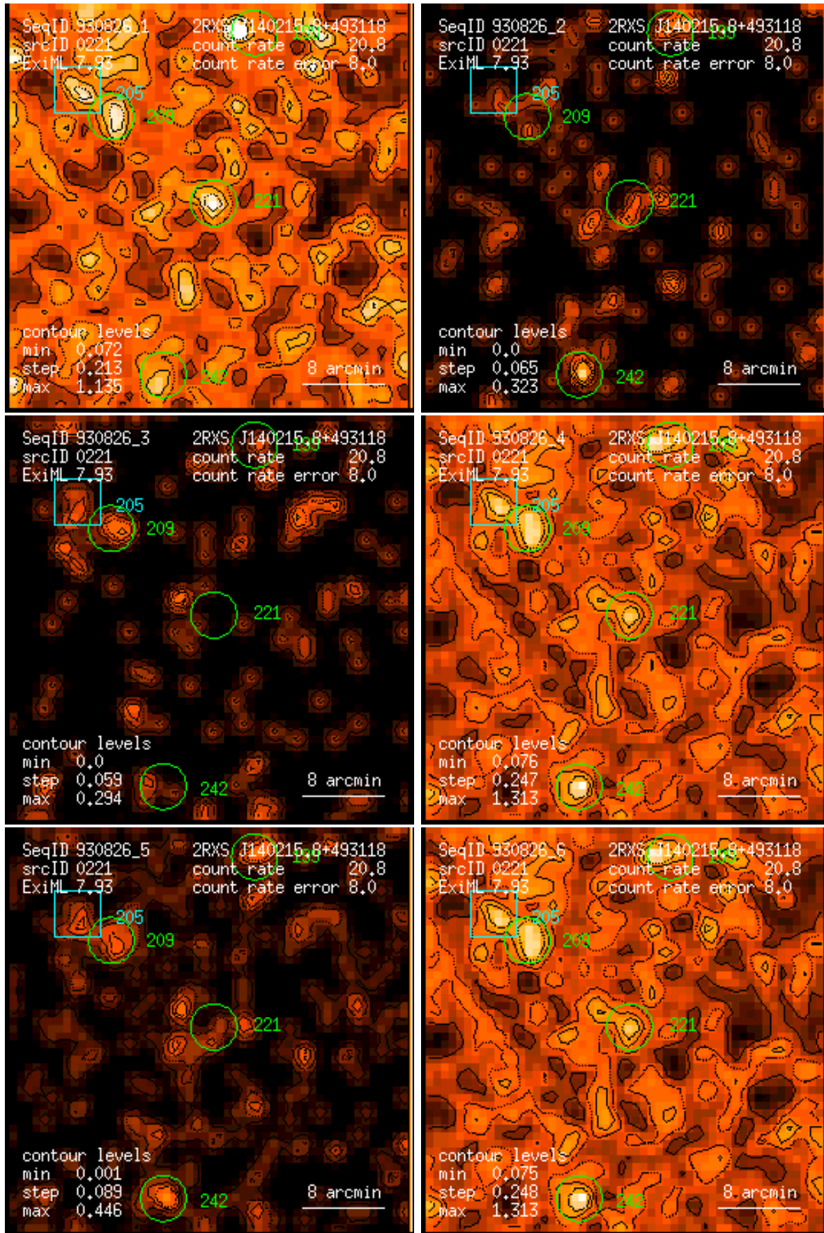
Figure 221: RASS 930826: detection 0221: band rate images, Gaussian filter: (1) PSPC channels 11 – 41, (2) 52 – 90, (3) 91 – 201, (4) 11 – 235, (5) 52 – 201, (6) 11 – 201. Broad band rates in counts/ks. Band rate contour levels in counts/ks/arcmin 2 .
