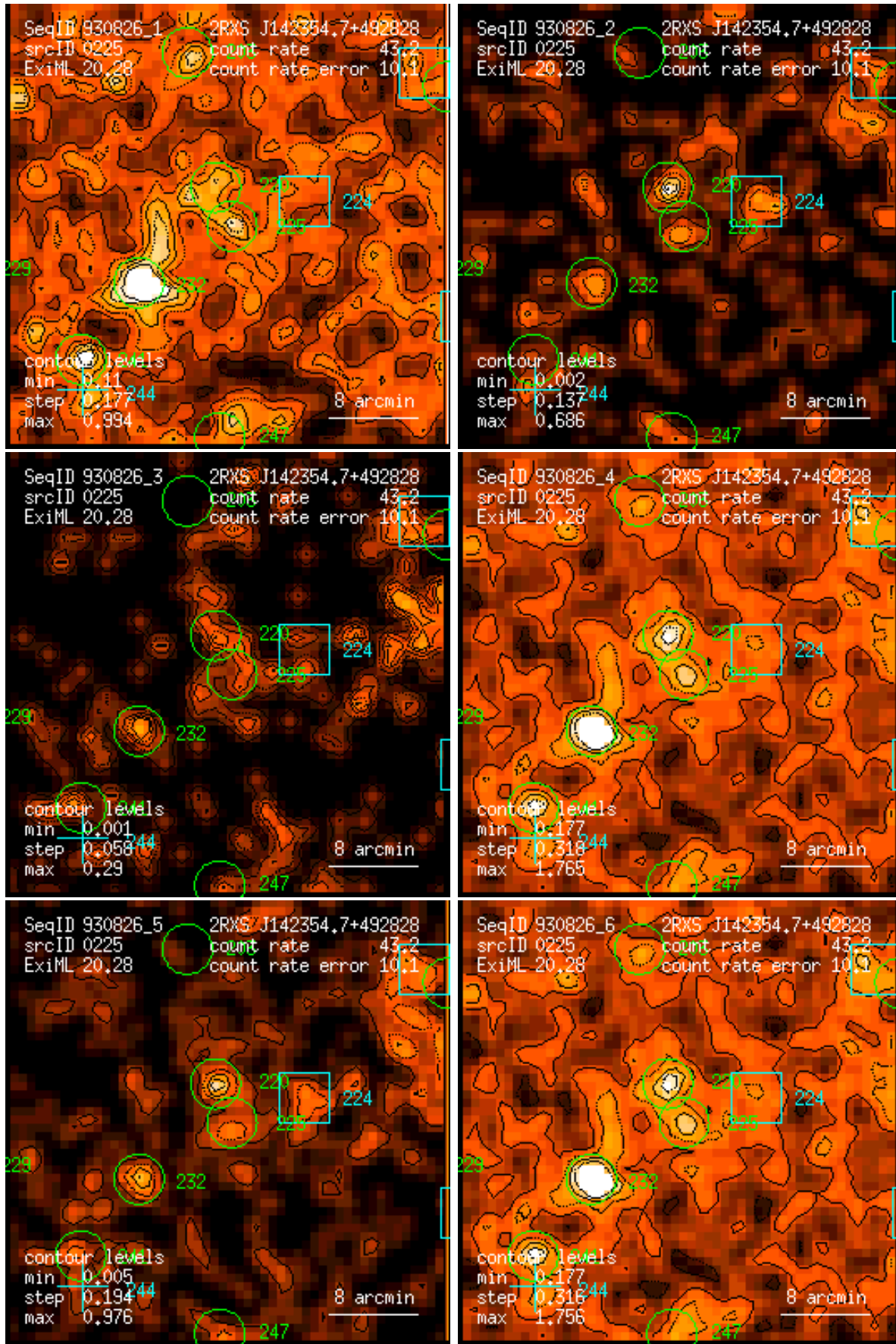
Figure 225: RASS 930826: detection 0225: band rate images, Gaussian filter: (1) PSPC channels 11 – 41, (2) 52 – 90, (3) 91 – 201, (4) 11 – 235, (5) 52 – 201, (6) 11 – 201. Broad band rates in counts/ks. Band rate contour levels in counts/ks/arcmin 2 .
