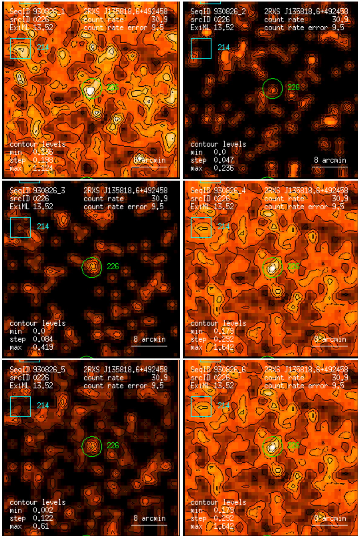
Figure 226: RASS 930826: detection 0226: band rate images, Gaussian filter: (1) PSPC channels 11 – 41, (2) 52 – 90, (3) 91 – 201, (4) 11 – 235, (5) 52 – 201, (6) 11 – 201. Broad band rates in counts/ks. Band rate contour levels in counts/ks/arcmin 2 .
