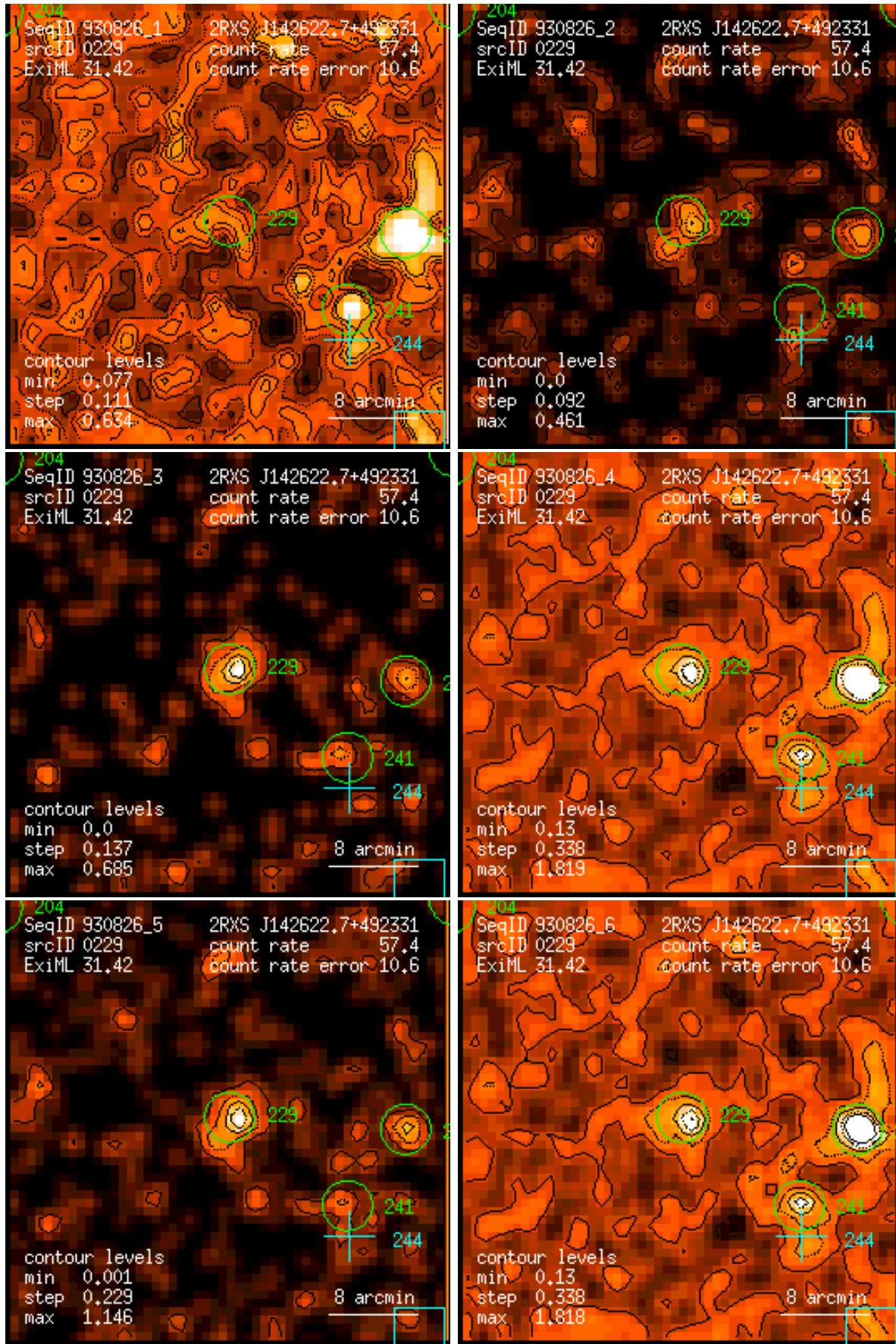
Figure 229: RASS 930826: detection 0229: band rate images, Gaussian filter: (1) PSPC channels 11 – 41, (2) 52 – 90, (3) 91 – 201, (4) 11 – 235, (5) 52 – 201, (6) 11 – 201. Broad band rates in counts/ks. Band rate contour levels in counts/ks/arcmin 2 .
