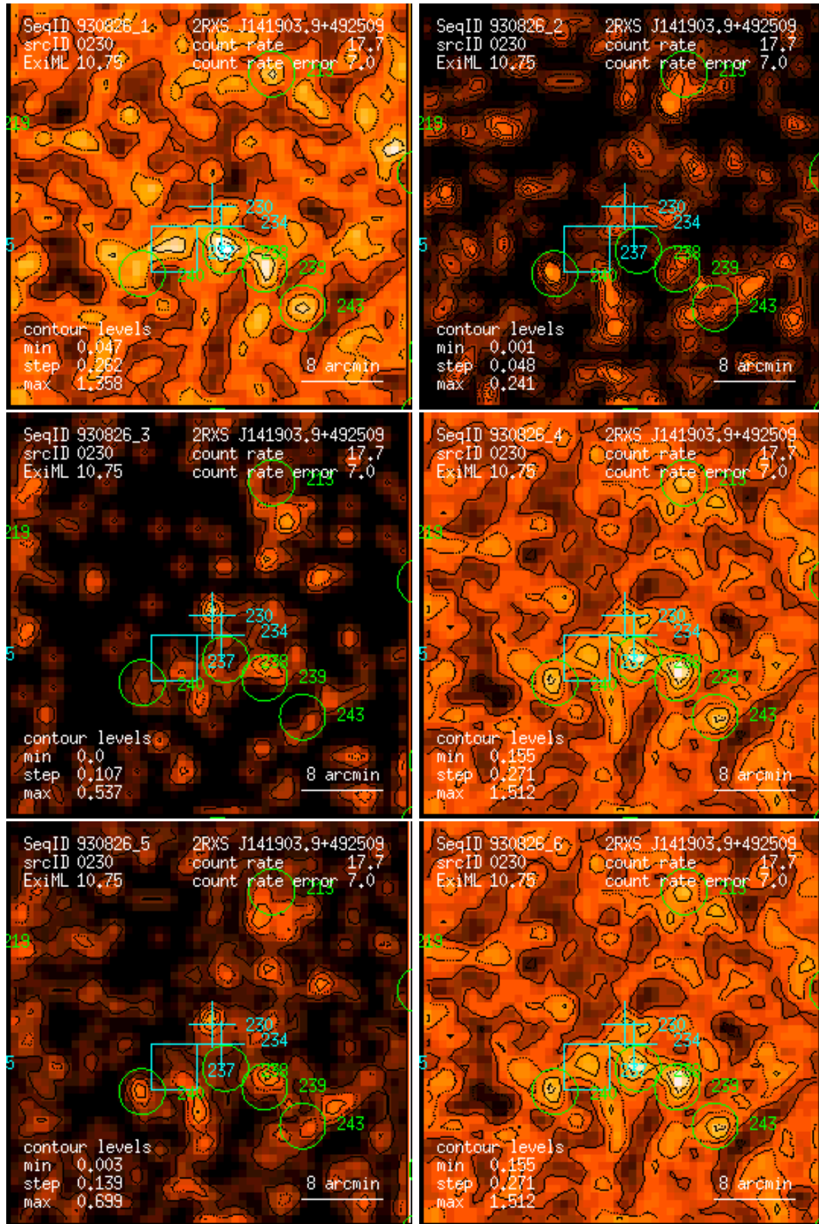
Figure 230: RASS 930826: detection 0230: band rate images, Gaussian filter: (1) PSPC channels 11 – 41, (2) 52 – 90, (3) 91 – 201, (4) 11 – 235, (5) 52 – 201, (6) 11 – 201. Broad band rates in counts/ks. Band rate contour levels in counts/ks/arcmin 2 .
