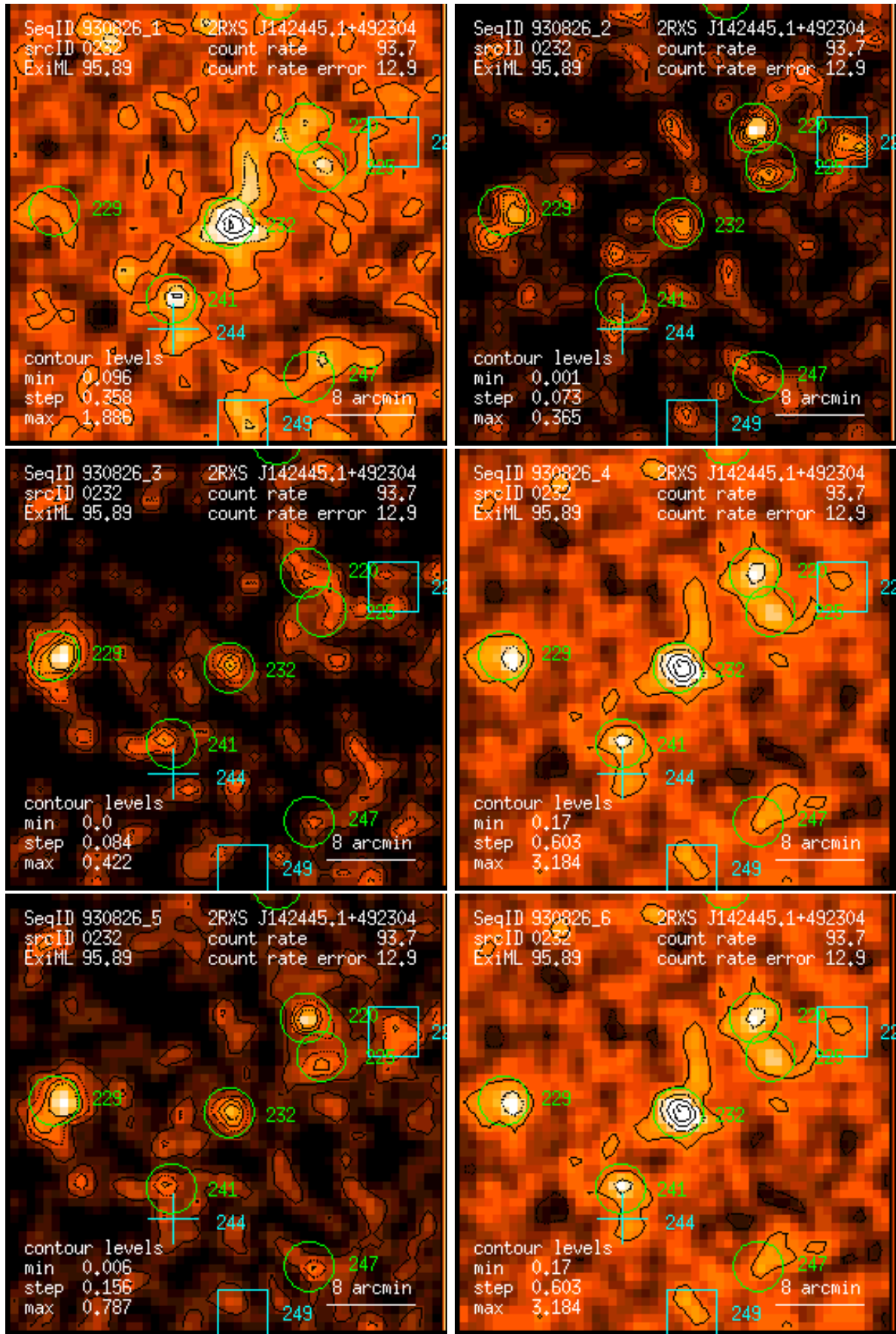
Figure 232: RASS 930826: detection 0232: band rate images, Gaussian filter: (1) PSPC channels 11 – 41, (2) 52 – 90, (3) 91 – 201, (4) 11 – 235, (5) 52 – 201, (6) 11 – 201. Broad band rates in counts/ks. Band rate contour levels in counts/ks/arcmin 2 .
