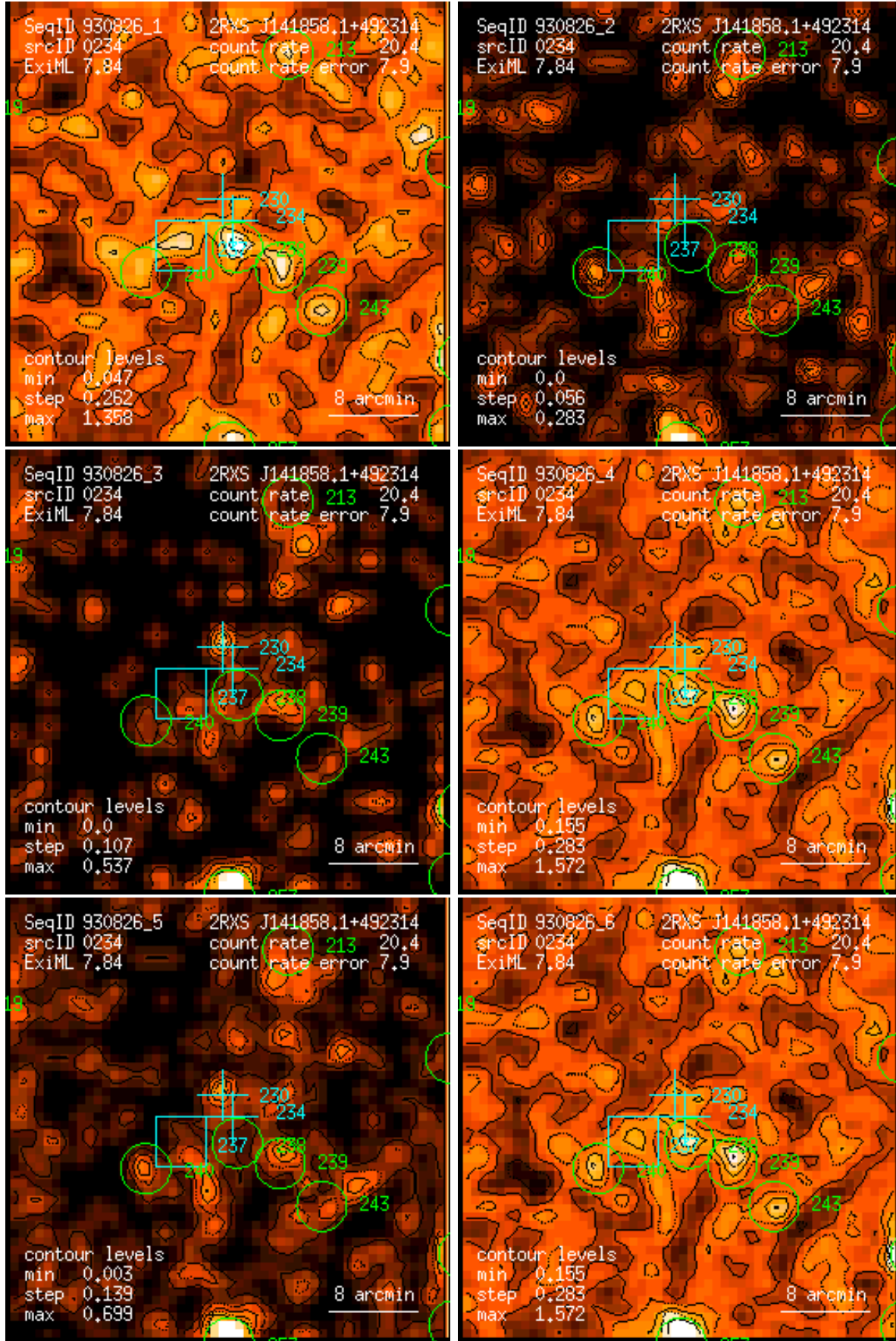
Figure 234: RASS 930826: detection 0234: band rate images, Gaussian filter: (1) PSPC channels 11 – 41, (2) 52 – 90, (3) 91 – 201, (4) 11 – 235, (5) 52 – 201, (6) 11 – 201. Broad band rates in counts/ks. Band rate contour levels in counts/ks/arcmin 2 .
