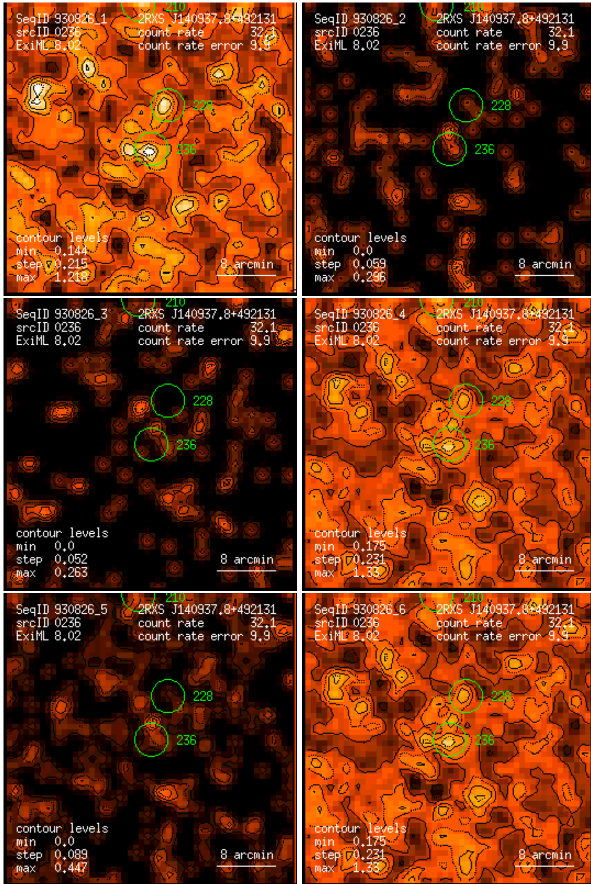
Figure 236: RASS 930826: detection 0236: band rate images, Gaussian filter: (1) PSPC channels 11 – 41, (2) 52 – 90, (3) 91 – 201, (4) 11 – 235, (5) 52 – 201, (6) 11 – 201. Broad band rates in counts/ks. Band rate contour levels in counts/ks/arcmin 2 .
