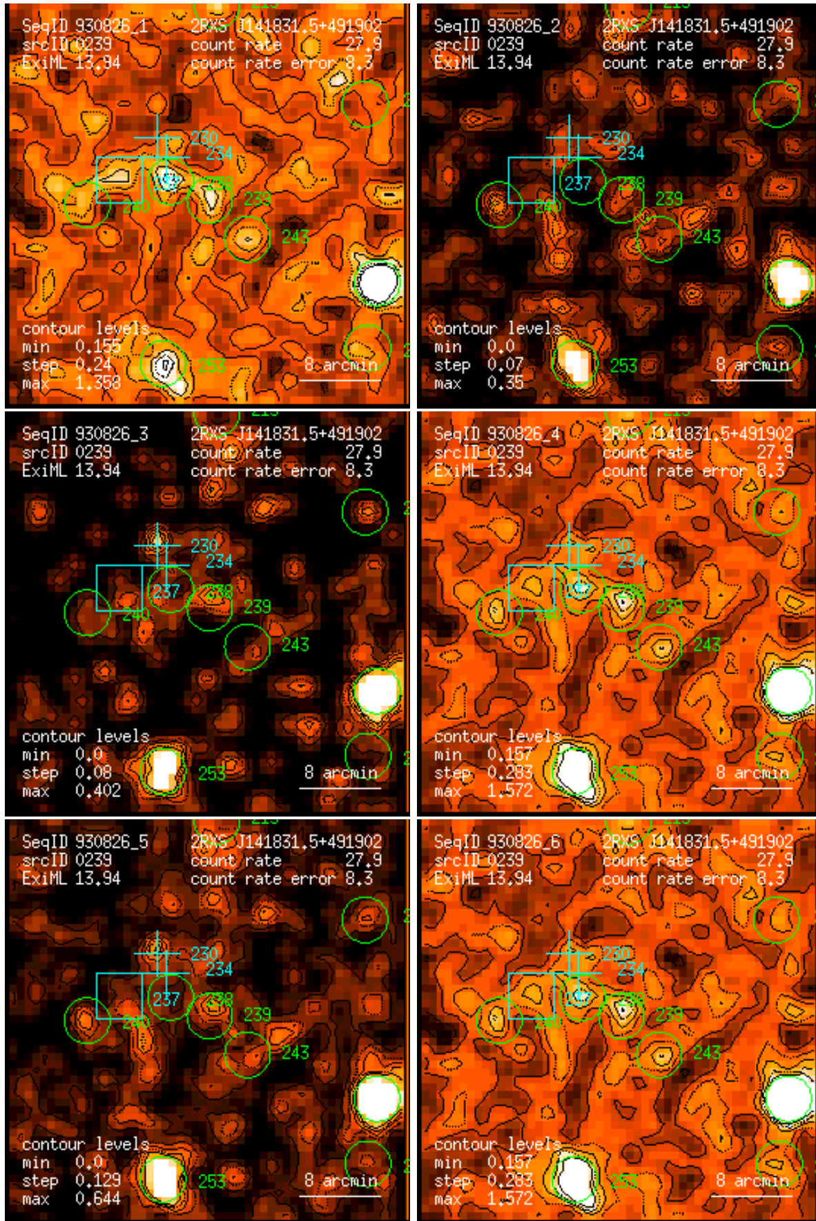
Figure 239: RASS 930826: detection 0239: band rate images, Gaussian filter: (1) PSPC channels 11 – 41, (2) 52 – 90, (3) 91 – 201, (4) 11 – 235, (5) 52 – 201, (6) 11 – 201. Broad band rates in counts/ks. Band rate contour levels in counts/ks/arcmin 2 .
