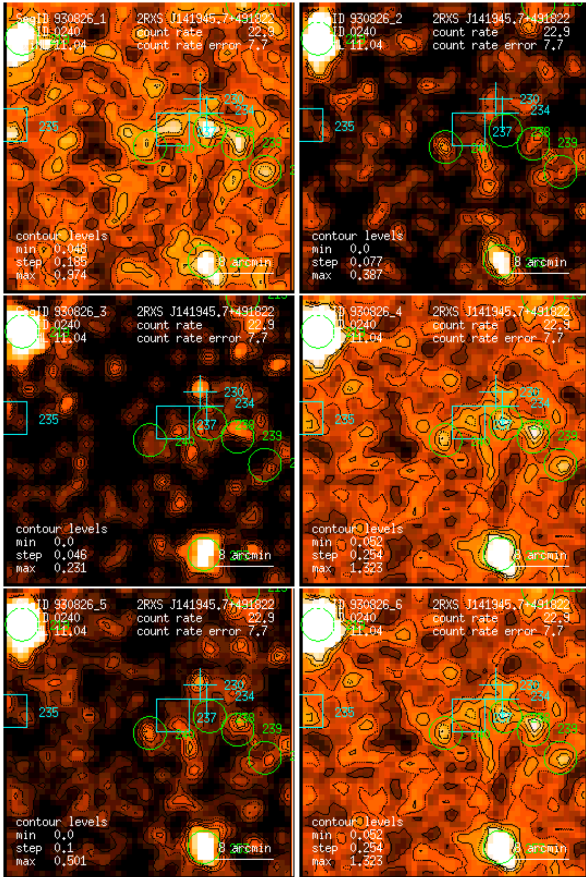
Figure 240: RASS 930826: detection 0240: band rate images, Gaussian filter: (1) PSPC channels 11 – 41, (2) 52 – 90, (3) 91 – 201, (4) 11 – 235, (5) 52 – 201, (6) 11 – 201. Broad band rates in counts/ks. Band rate contour levels in counts/ks/arcmin 2 .
