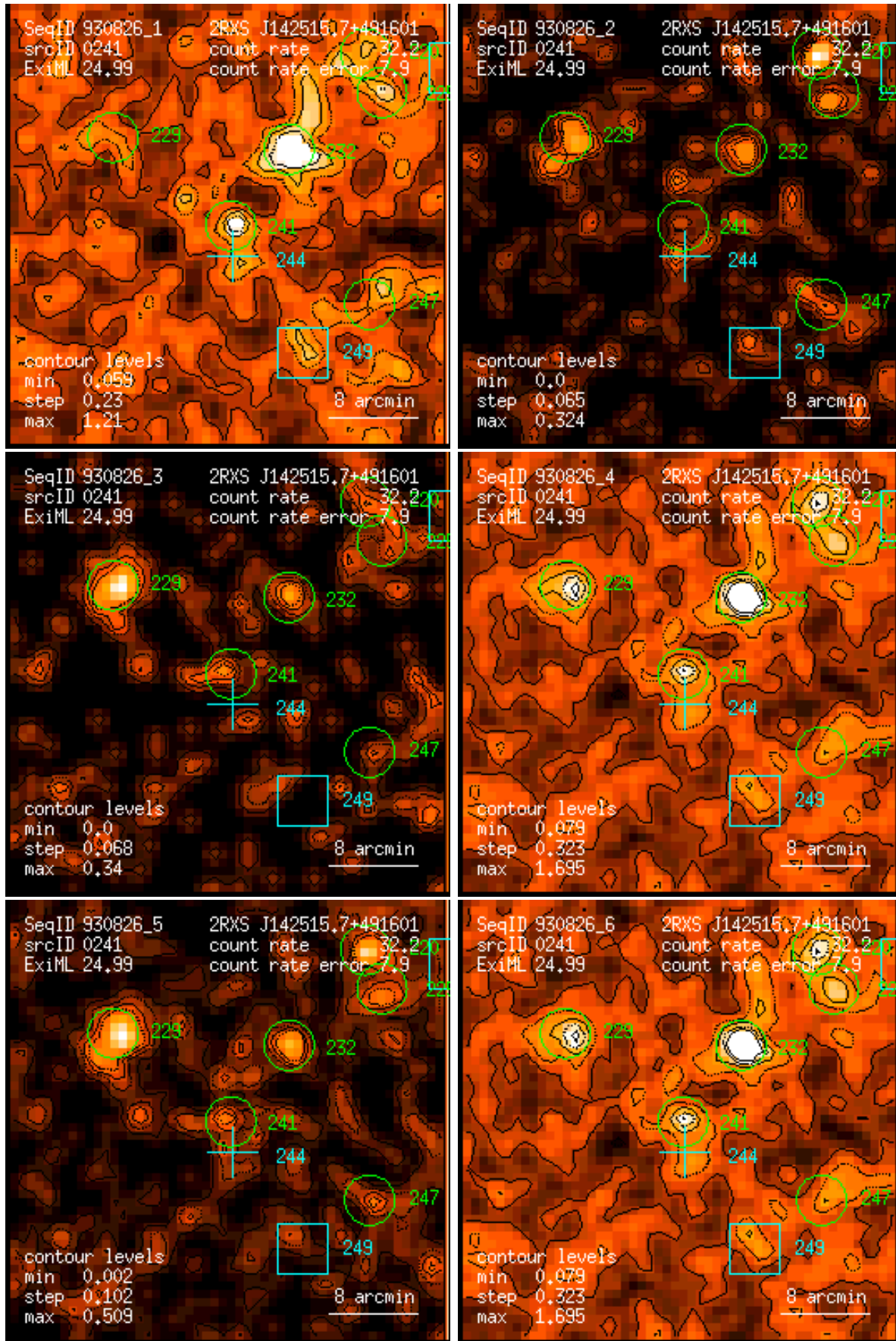
Figure 241: RASS 930826: detection 0241: band rate images, Gaussian filter: (1) PSPC channels 11 – 41, (2) 52 – 90, (3) 91 – 201, (4) 11 – 235, (5) 52 – 201, (6) 11 – 201. Broad band rates in counts/ks. Band rate contour levels in counts/ks/arcmin 2 .
