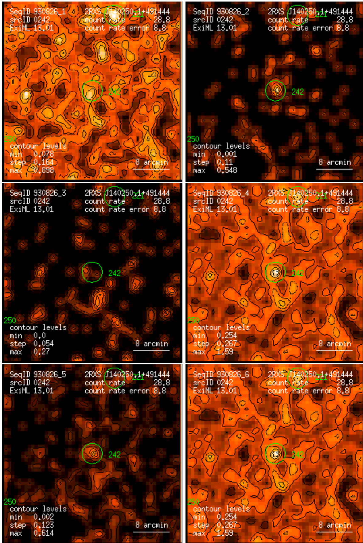
Figure 242: RASS 930826: detection 0242: band rate images, Gaussian filter: (1) PSPC channels 11 – 41, (2) 52 – 90, (3) 91 – 201, (4) 11 – 235, (5) 52 – 201, (6) 11 – 201. Broad band rates in counts/ks. Band rate contour levels in counts/ks/arcmin 2 .
