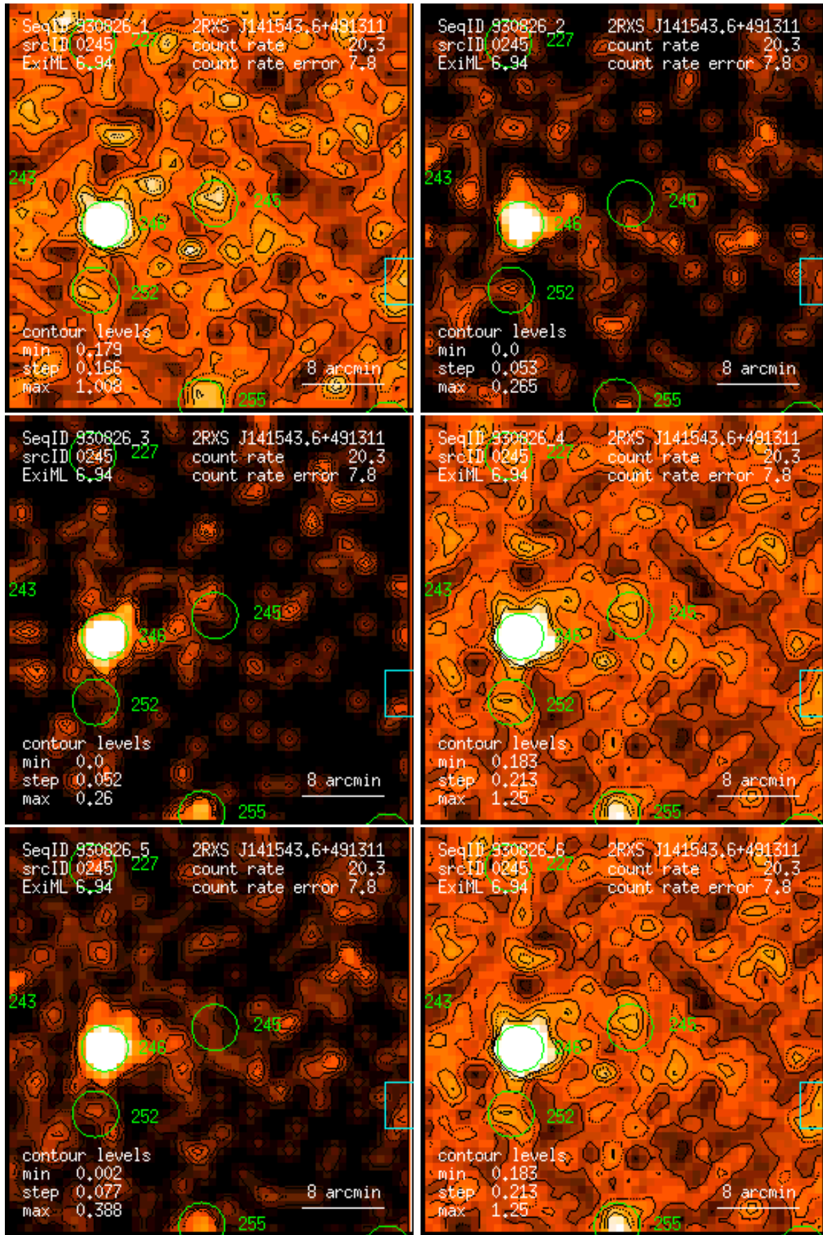
Figure 245: RASS 930826: detection 0245: band rate images, Gaussian filter: (1) PSPC channels 11 – 41, (2) 52 – 90, (3) 91 – 201, (4) 11 – 235, (5) 52 – 201, (6) 11 – 201. Broad band rates in counts/ks. Band rate contour levels in counts/ks/arcmin 2 .
