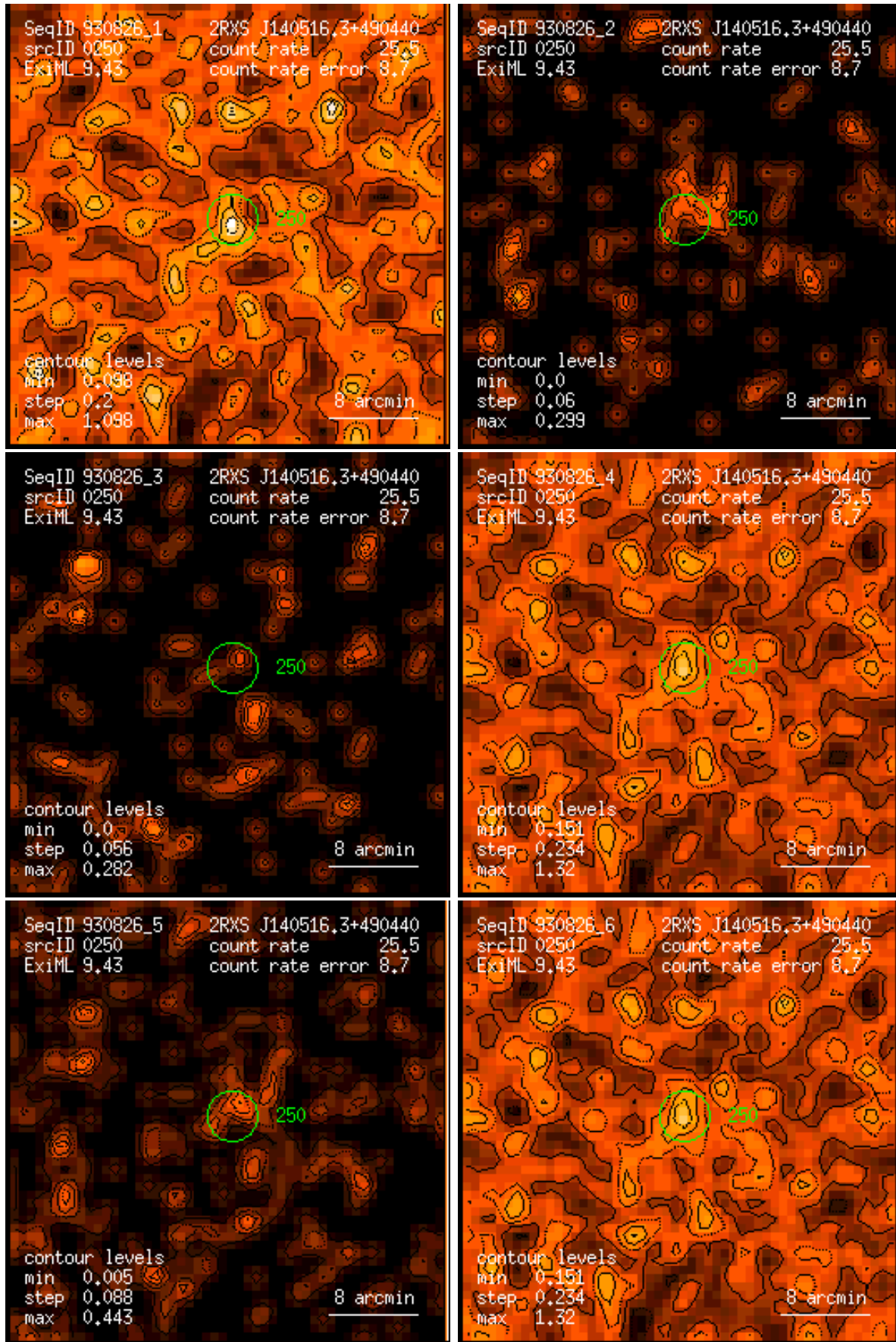
Figure 250: RASS 930826: detection 0250: band rate images, Gaussian filter: (1) PSPC channels 11 – 41, (2) 52 – 90, (3) 91 – 201, (4) 11 – 235, (5) 52 – 201, (6) 11 – 201. Broad band rates in counts/ks. Band rate contour levels in counts/ks/arcmin 2 .
