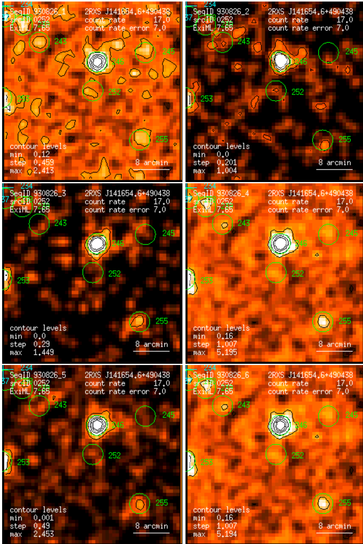
Figure 252: RASS 930826: detection 0252: band rate images, Gaussian filter: (1) PSPC channels 11 – 41, (2) 52 – 90, (3) 91 – 201, (4) 11 – 235, (5) 52 – 201, (6) 11 – 201. Broad band rates in counts/ks. Band rate contour levels in counts/ks/arcmin 2 .
