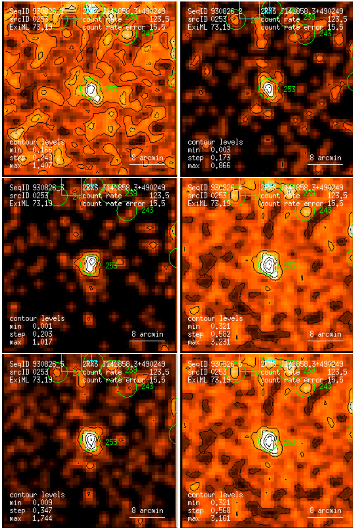
Figure 253: RASS 930826: detection 0253: band rate images, Gaussian filter: (1) PSPC channels 11 – 41, (2) 52 – 90, (3) 91 – 201, (4) 11 – 235, (5) 52 – 201, (6) 11 – 201. Broad band rates in counts/ks. Band rate contour levels in counts/ks/arcmin 2 .
