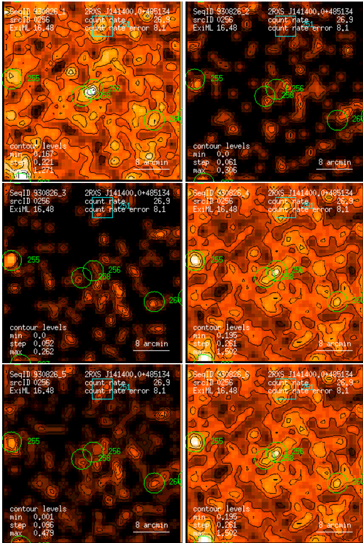
Figure 256: RASS 930826: detection 0256: band rate images, Gaussian filter: (1) PSPC channels 11 – 41, (2) 52 – 90, (3) 91 – 201, (4) 11 – 235, (5) 52 – 201, (6) 11 – 201. Broad band rates in counts/ks. Band rate contour levels in counts/ks/arcmin 2 .
