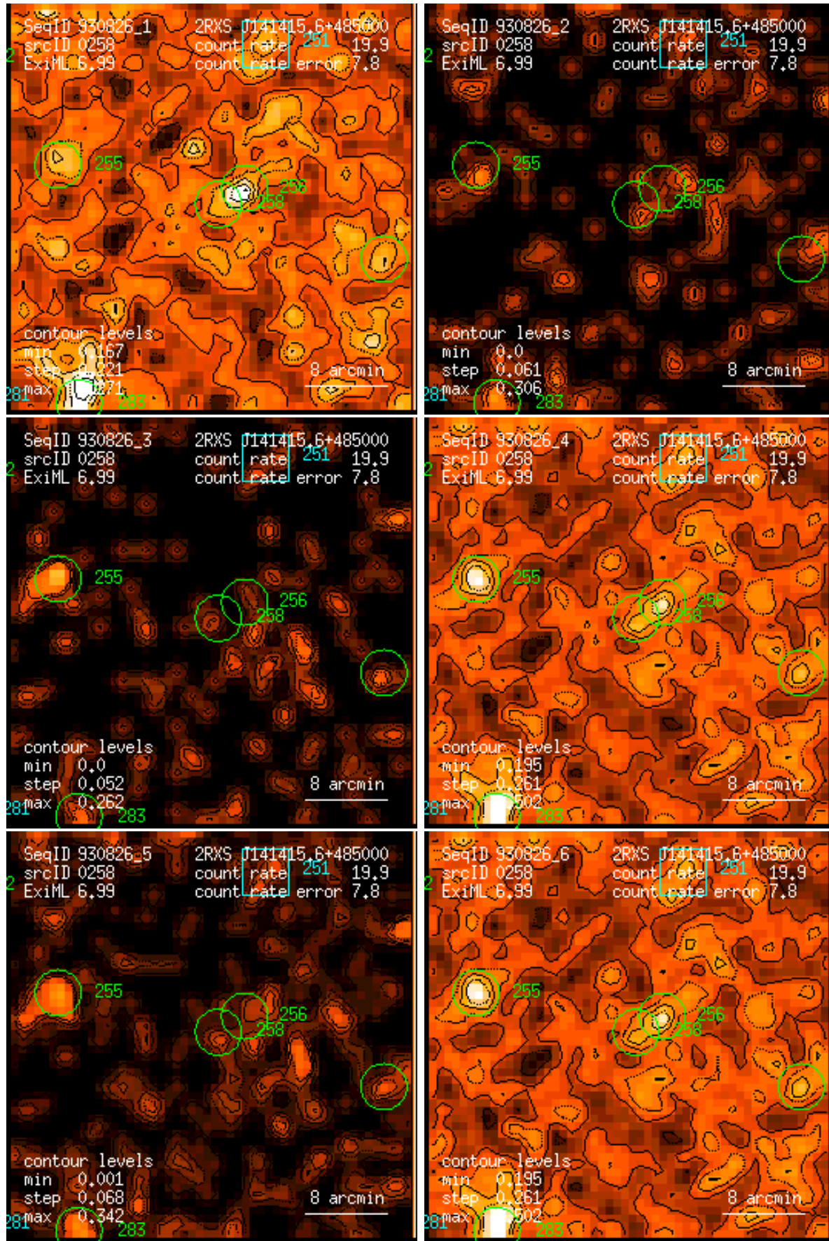
Figure 258: RASS 930826: detection 0258: band rate images, Gaussian filter: (1) PSPC channels 11 – 41, (2) 52 – 90, (3) 91 – 201, (4) 11 – 235, (5) 52 – 201, (6) 11 – 201. Broad band rates in counts/ks. Band rate contour levels in counts/ks/arcmin 2 .
