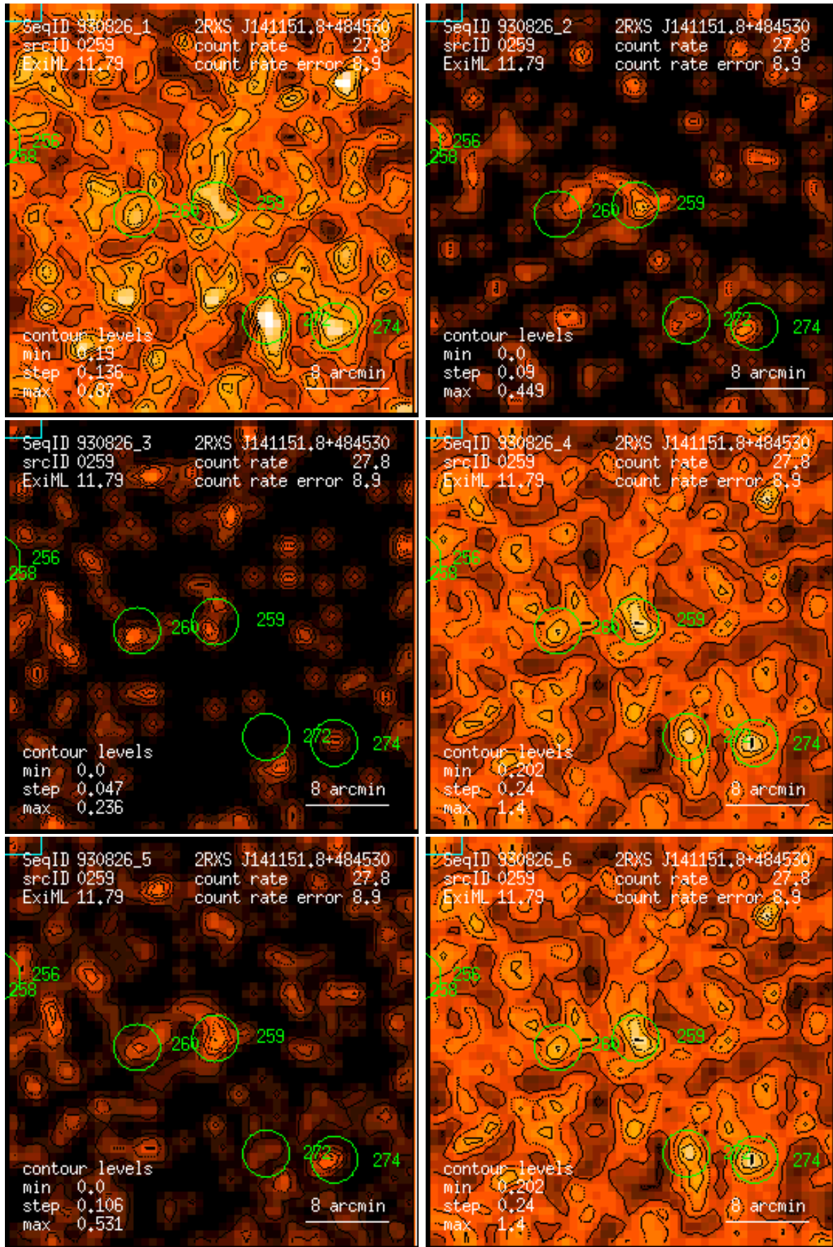
Figure 259: RASS 930826: detection 0259: band rate images, Gaussian filter: (1) PSPC channels 11 – 41, (2) 52 – 90, (3) 91 – 201, (4) 11 – 235, (5) 52 – 201, (6) 11 – 201. Broad band rates in counts/ks. Band rate contour levels in counts/ks/arcmin 2 .
