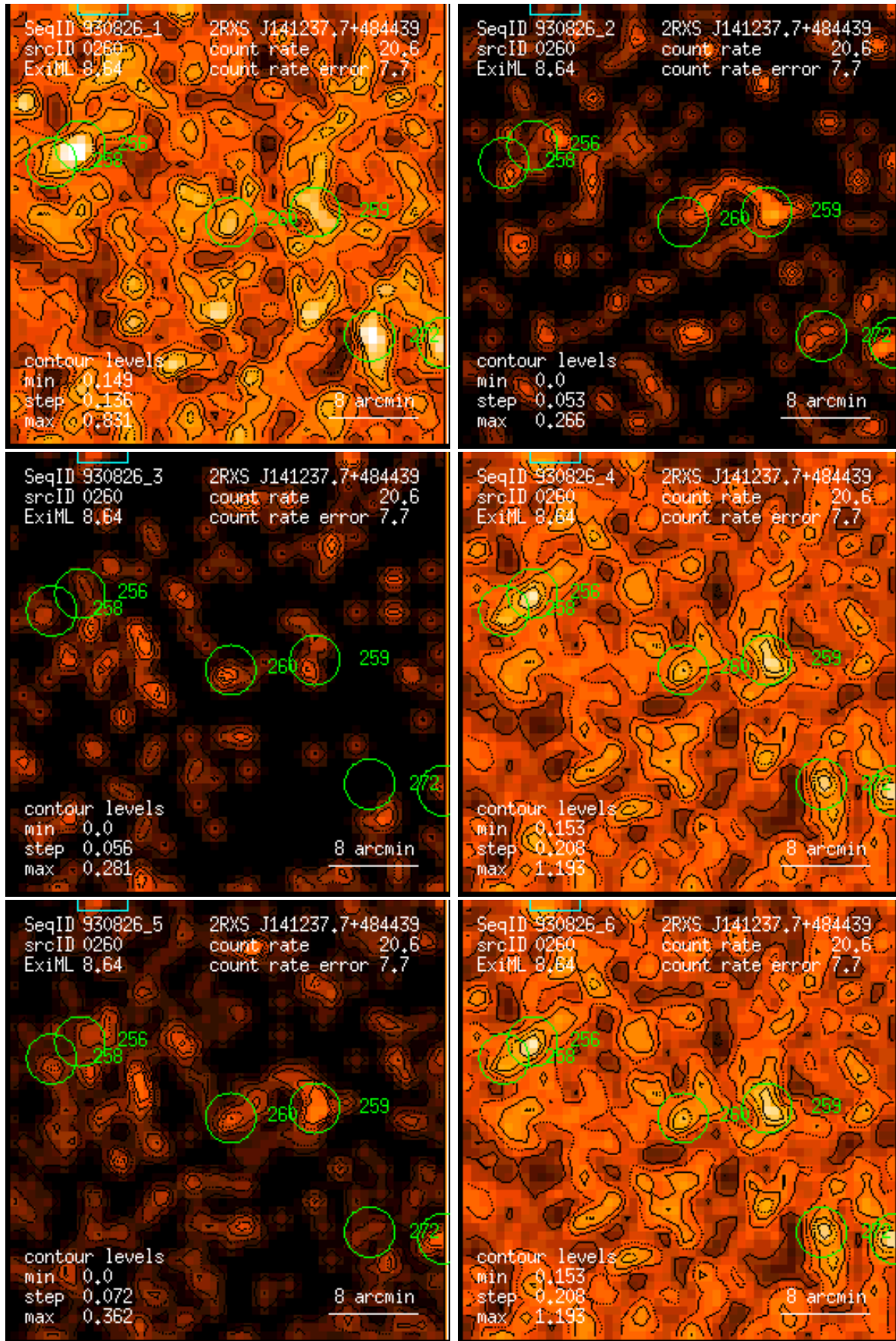
Figure 260: RASS 930826: detection 0260: band rate images, Gaussian filter: (1) PSPC channels 11 – 41, (2) 52 – 90, (3) 91 – 201, (4) 11 – 235, (5) 52 – 201, (6) 11 – 201. Broad band rates in counts/ks. Band rate contour levels in counts/ks/arcmin 2 .
