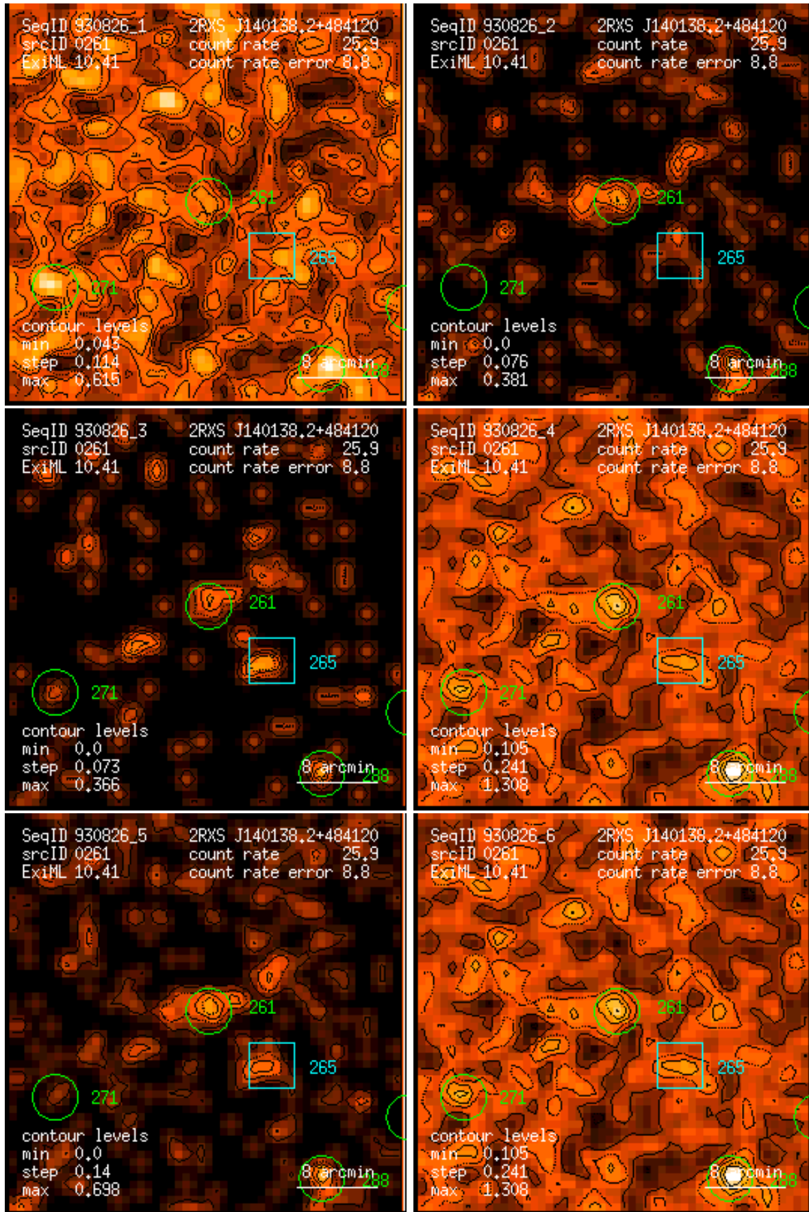
Figure 261: RASS 930826: detection 0261: band rate images, Gaussian filter: (1) PSPC channels 11 – 41, (2) 52 – 90, (3) 91 – 201, (4) 11 – 235, (5) 52 – 201, (6) 11 – 201. Broad band rates in counts/ks. Band rate contour levels in counts/ks/arcmin 2 .
