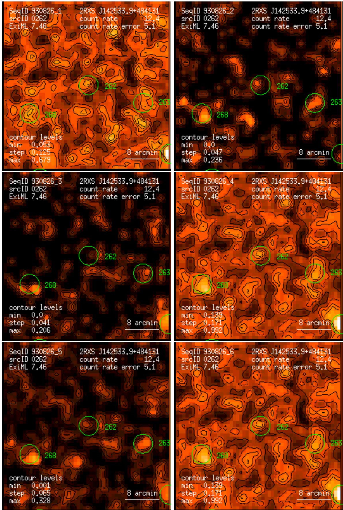
Figure 262: RASS 930826: detection 0262: band rate images, Gaussian filter: (1) PSPC channels 11 – 41, (2) 52 – 90, (3) 91 – 201, (4) 11 – 235, (5) 52 – 201, (6) 11 – 201. Broad band rates in counts/ks. Band rate contour levels in counts/ks/arcmin 2 .
